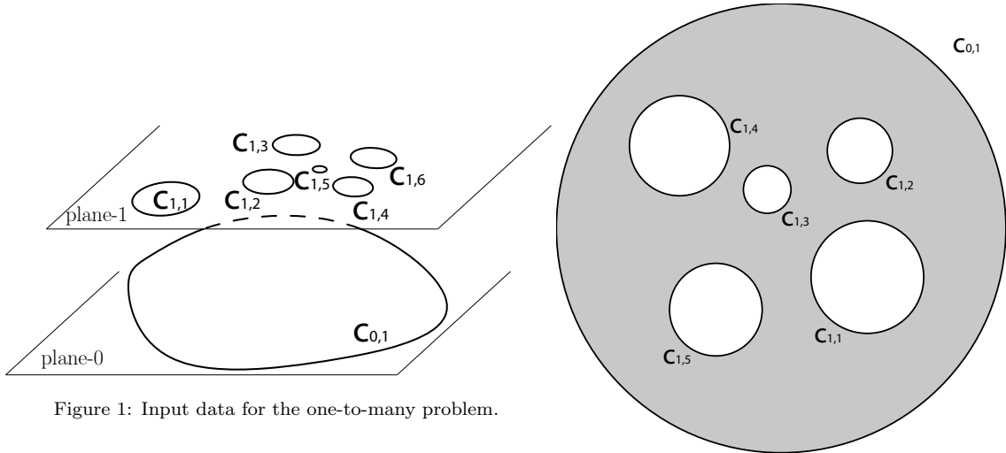
Figure 2: Hollowed disc corresponding to interpolating surface. Surface borders correspond to contours on plane-0 ( C_{0,1} ) and plane-1 ( C_{1,i} , i = 1, \dots, 5 ).
