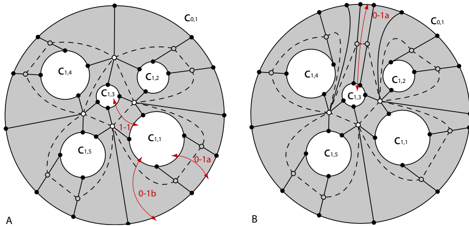
Figure 3: Disc decompositions.
