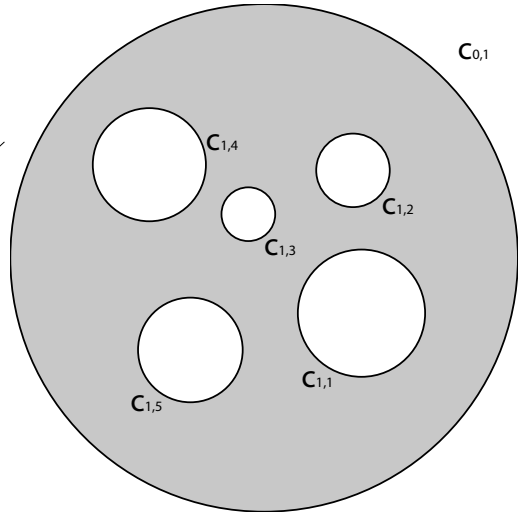
Figure 2: Hollowed disc corresponding to interpolating surface. Surface borders correspond to contours on plane-0 ( C_{0,1} ) and plane-1 ( C_{1,i} , i = 1, \dots, 5 ).
