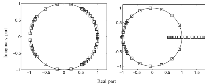
Fig. 20 Stability analysis of mode (1,15): a) FEP, in which a solid (dashed) line indicates stability (instability); and b) unit circle and Floquet multipliers, which are represented by squares.
