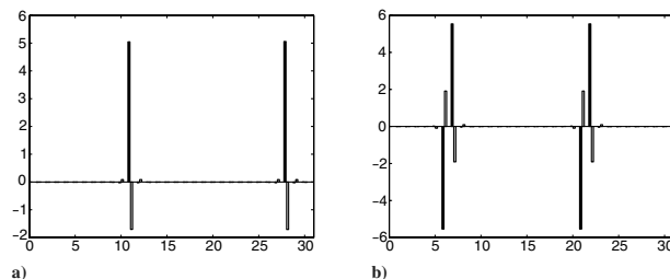
Fig. 18 Bifurcation of the mode pair (1,14).
