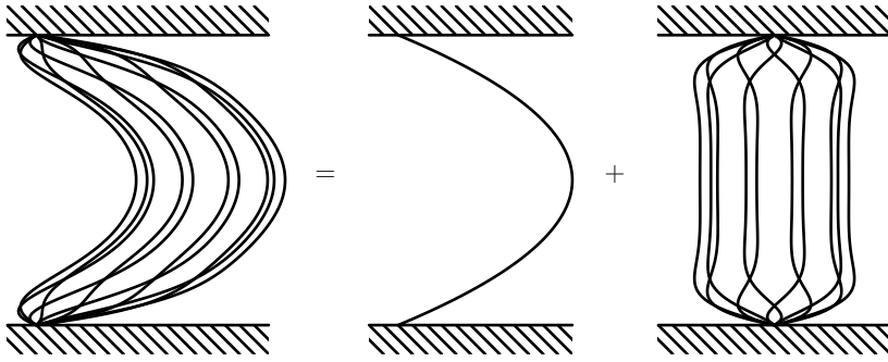
FIGURE 1. Snapshots of typical base-flow profile associated with a flow rate of the form Q(t)/Q^{(0)} = 1 + \tilde{Q} \cos \Omega t . In this example, Wo = 10 and \tilde{Q} = 0.6 and ten profiles over one complete pulsation cycle are shown.
