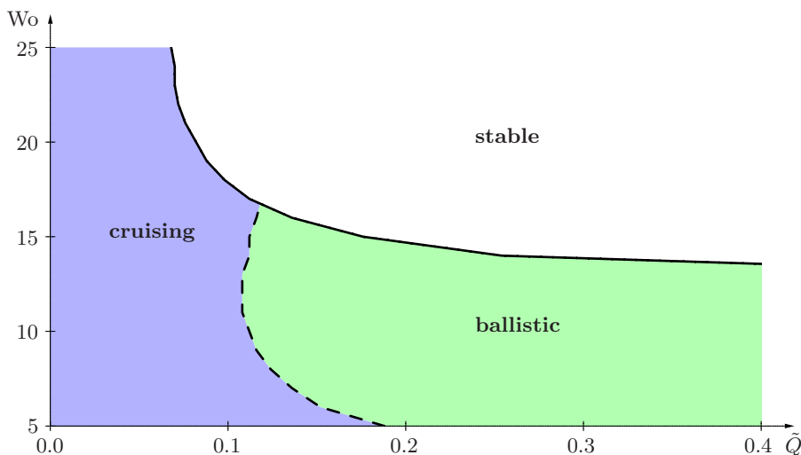
FIGURE 19. Phase diagram of the flow dynamics for \text{Re} = 10000 and \alpha_1 = 2 . A cruising regime prevails at low base-flow modulation amplitudes \tilde{Q} . At larger \tilde{Q} , to the right of the dashed curve, a ballistic regime takes over. Above the black curve, the pulsating base flow is linearly stable.
