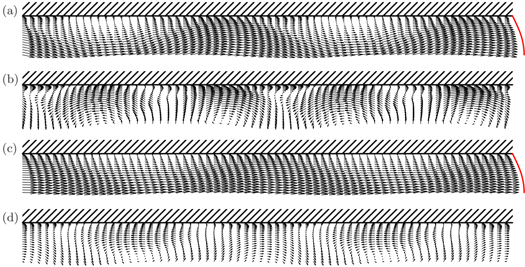
FIGURE 12. Snapshots of velocity fields in cruising nonlinear regime over two wavelengths with \alpha_1 = 2 at \text{Re} = 10000 , \text{Wo} = 10 and \tilde{Q} = 0.08 : (a) total velocity at t/T = 29.5 , (b) perturbation velocity at t/T = 29.5 , (c) total velocity at t/T = 30.0 , (d) perturbation velocity at t/T = 30.0 . Solid curves to the right of (a) and (c) indicate base-flow profile prevailing at same instant.
