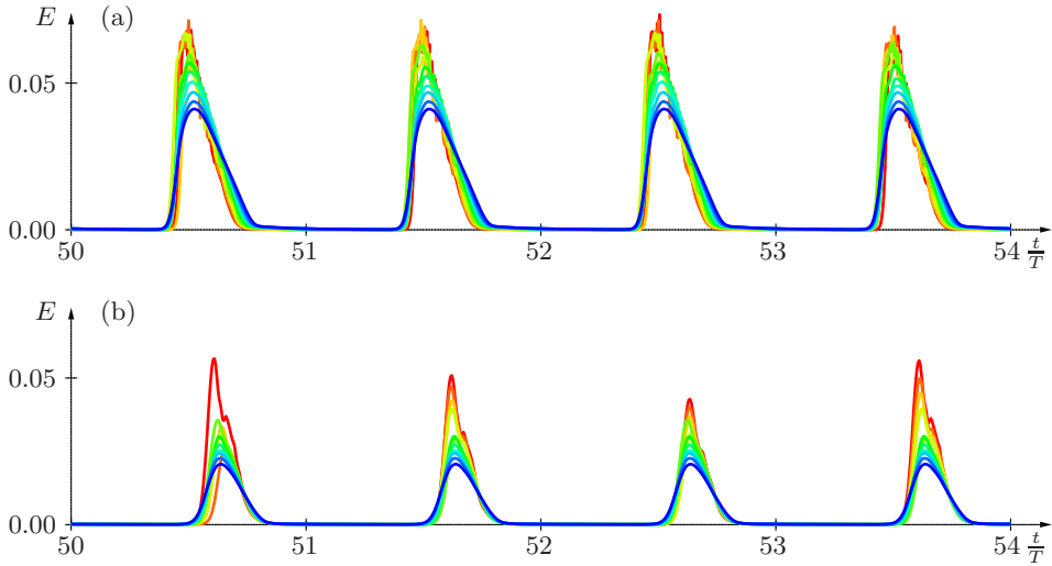
FIGURE 18. Temporal evolution of perturbation energy in fully developed regime at (a) Wo = 7 , (b) Wo = 10 , for \tilde{Q} = 0.20 (dark blue), 0.22, \dots, 0.38, 0.40 (red) and \alpha_1 = 2 , Re = 10000 . The maximum energy of the nonlinear bursts increases with \tilde{Q} and, at larger values of \tilde{Q} , successive peaks culminate at slightly different levels.
