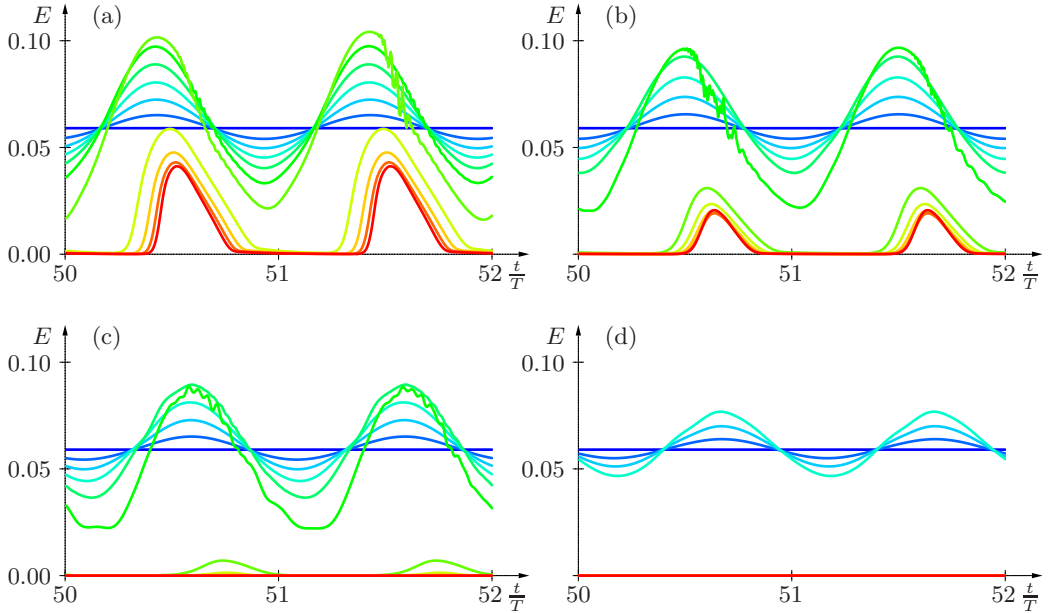
FIGURE 17. Temporal evolution of perturbation energy in fully developed regime at (a) Wo = 7 , (b) Wo = 10 , (c) Wo = 15 , (d) Wo = 20 , for \tilde{Q} = 0.00 (horizontal line), 0.02, 0.04, \dots , 0.20 and \alpha_1 = 2 , Re = 10000 .
