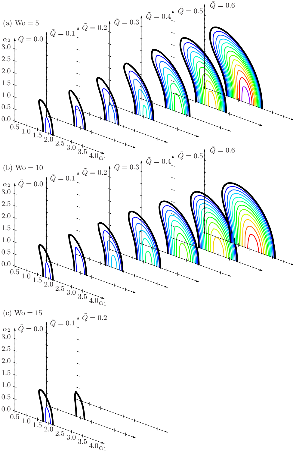
FIGURE 9. Isolines of temporal growth rate \omega_i in the (\alpha_1, \alpha_2) -wavevector plane for \tilde{Q} = 0.0, 0.1, \dots, 0.6 at (a) Wo = 5 , (b) Wo = 10 , (c) Wo = 15 . Thick black lines correspond to the marginal curve \omega_i = 0 and thin coloured lines to positive growth rates \omega_i = 0.005, 0.010, 0.015, \dots
