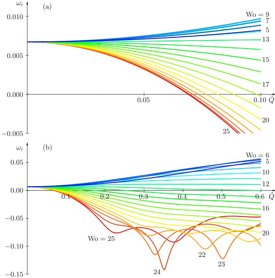
FIGURE 5. Linear temporal growth rate at \text{Re} = 10000 and \alpha_1 = 2 for 0 \leq \tilde{Q} \leq 0.6 and \text{Wo} = 5, 6, \dots, 25 .
