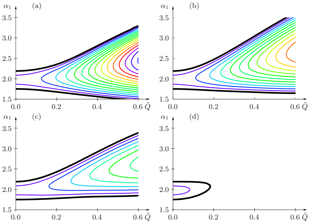
FIGURE 8. Isolines of linear temporal growth rate for two-dimensional perturbations in (\alpha_1, \tilde{Q}) -plane at \text{Re} = 10000 and (a) \text{Wo} = 6 , (b) \text{Wo} = 10 , (c) \text{Wo} = 12 , (d) \text{Wo} = 15 . Thick black lines correspond to the marginal curve \omega_i = 0 and thin coloured lines to positive growth rates \omega_i = 0.005, 0.010, 0.015, \dots
