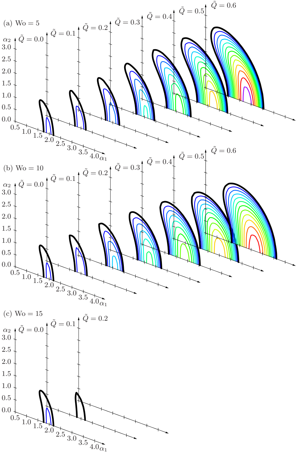
FIGURE 9. Isolines of temporal growth rate \omega_i in the (\alpha_1, \alpha_2) -wavevector plane for \tilde{Q} = 0.0, 0.1, \dots, 0.6 at (a) Wo = 5 , (b) Wo = 10 , (c) Wo = 15 . Thick black lines correspond to the marginal curve \omega_i = 0 and thin coloured lines to positive growth rates \omega_i = 0.005, 0.010, 0.015, \dots
