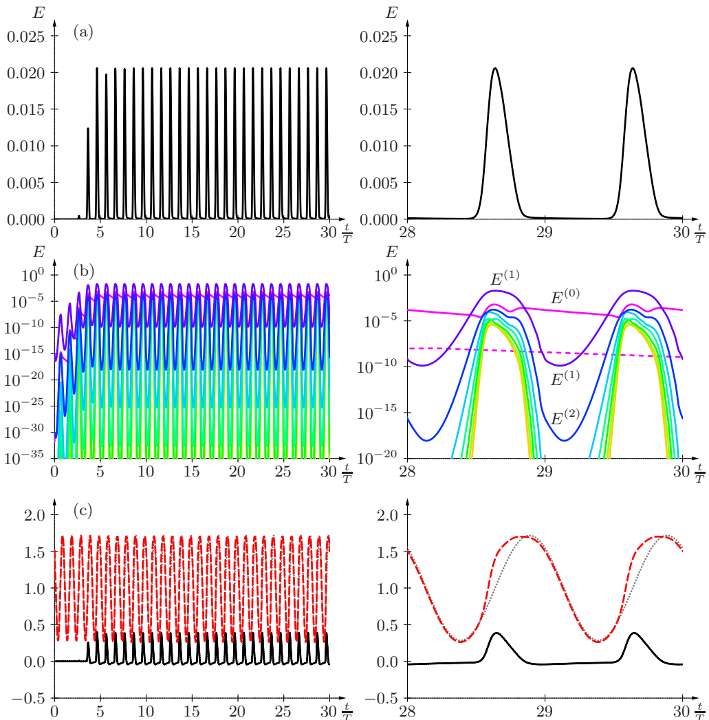
FIGURE 14. “Ballistic” nonlinear regime resulting from modulated exponential growth of small-amplitude initial perturbation with \alpha_1 = 2 at \text{Re} = 10000 , \text{Wo} = 10 and \tilde{Q} = 0.2 . (a) Total perturbation energy. (b) Energy of each spatial Fourier component. (c) Spatially averaged wall shear stress of perturbation (black solid), total (red dashed) and base (grey dotted) fields relative to steady Poiseuille flow value.
