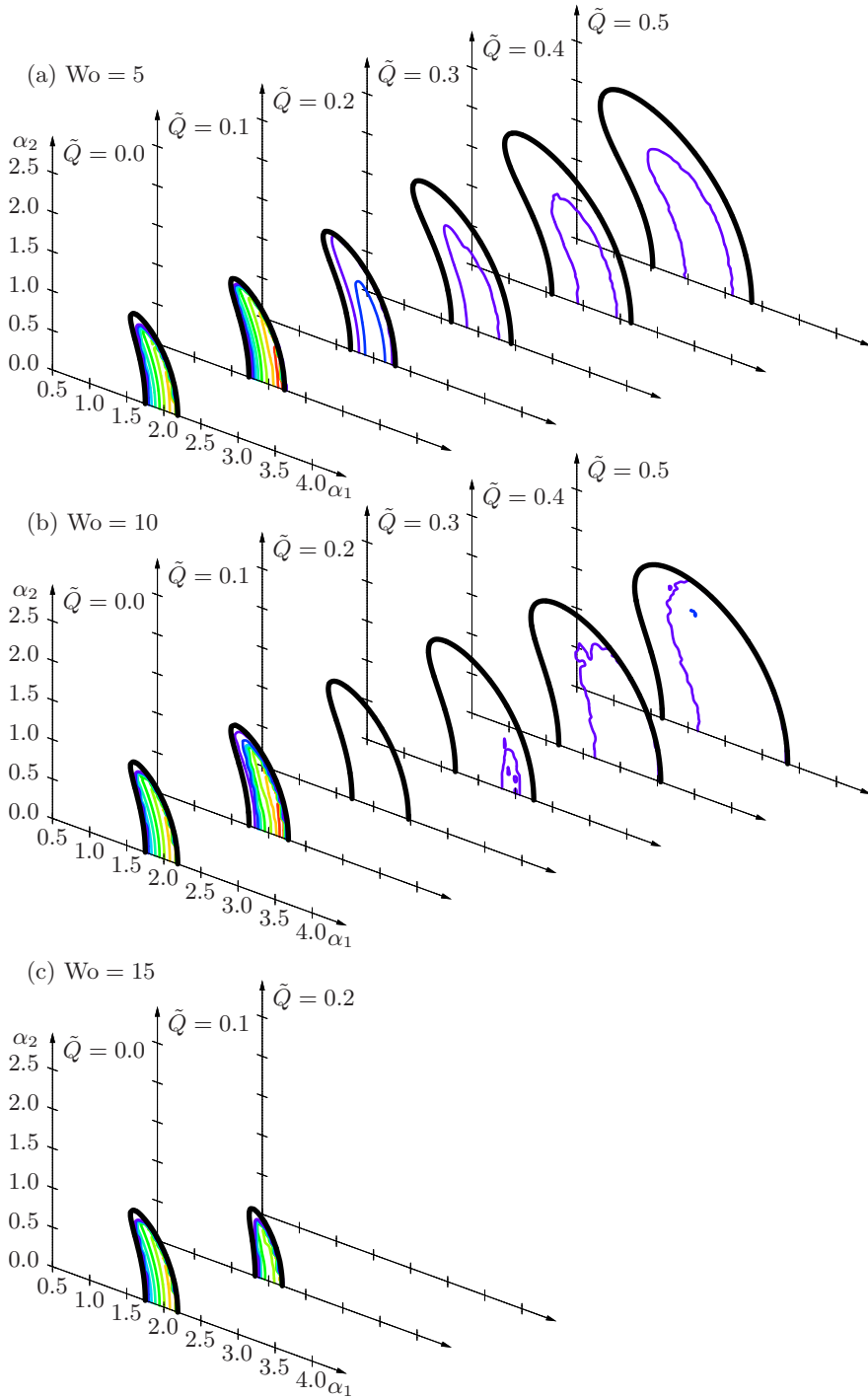
FIGURE 21. Isolines of average energy levels for three-dimensional nonlinear solutions in the (\alpha_1, \alpha_2) -wavevector plane for \tilde{Q} = 0.0, 0.1, \dots, 0.5 at (a) Wo = 5 , (b) Wo = 10 , (c) Wo = 15 and Re = 10000 . Color isolines correspond to E = 0.01, 0.02, 0.03, \dots , and the thick black curve represents the neutral boundary.
