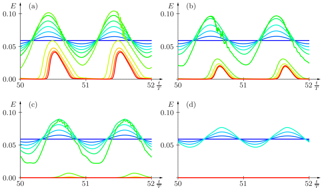
FIGURE 17. Temporal evolution of perturbation energy in fully developed regime at (a) Wo = 7 , (b) Wo = 10 , (c) Wo = 15 , (d) Wo = 20 , for \tilde{Q} = 0.00 (horizontal line), 0.02, 0.04, \dots, 0.20 and \alpha_1 = 2 , Re = 10000 .
