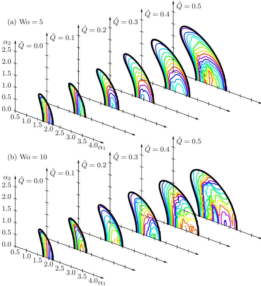
FIGURE 23. Isolines of maximum local WSS levels for three-dimensional nonlinear solutions in the (\alpha_1, \alpha_2) -wavevector plane for \tilde{Q} = 0.0, 0.1, \dots, 0.5 at (a) Wo = 5 , (b) Wo = 10 and Re = 10000 . Color isolines correspond to WSS = 0.5, 1.0, 1.5, \dots , relative to Poiseuille value, and the thick black curve represents the neutral boundary.
