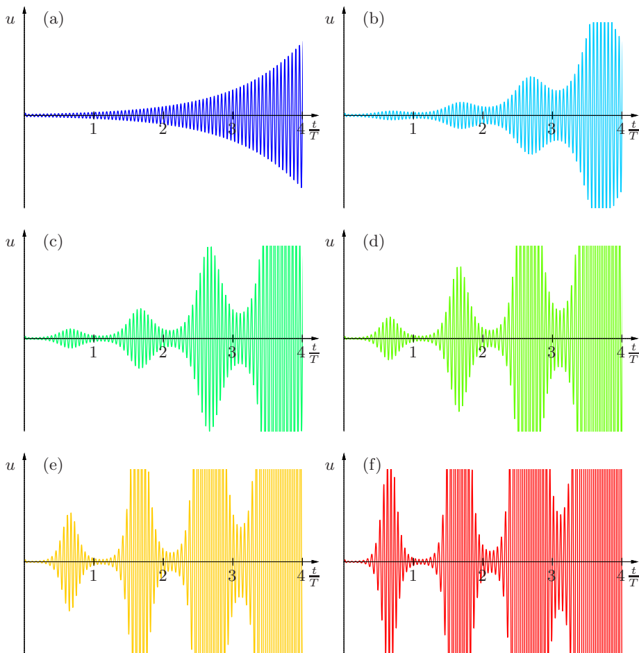
FIGURE 2. Temporal evolution of a small-amplitude perturbation with \alpha_1 = 2 at \text{Re} = 10000 and \text{Wo} = 10 . Perturbation velocity time series for base flow with (a) \tilde{Q} = 0 (Poiseuille flow), (b) \tilde{Q} = 0.02 , (c) \tilde{Q} = 0.04 , (d) \tilde{Q} = 0.06 , (e) \tilde{Q} = 0.08 and (f) \tilde{Q} = 0.10 over 4 base-flow pulsation cycles. In this linear dynamics, the velocity scale is arbitrary but identical for all cases shown, and the same initial perturbation has been used throughout to trigger the perturbation.
