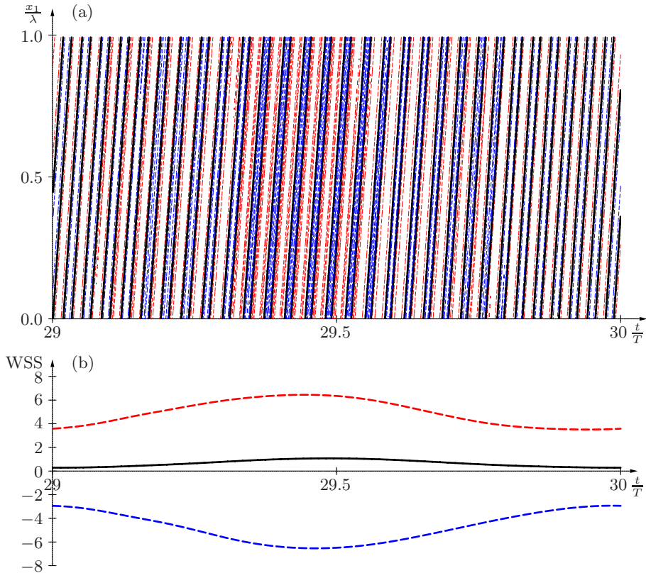
FIGURE 13. (a) Spatio-temporal pattern of the perturbation WSS in cruising regime over one streamwise wavelength \lambda = 2\pi/\alpha_1 and one pulsation period. WSS values are relative to a steady Poiseuille flow at the same Reynolds number, and thick solid black isoline corresponding to WSS = 0 separates thin dashed red (resp. blue) isolines corresponding to levels WSS = 2, 4, 6 (resp. WSS = -2, -4, -6 ). (b) Instantaneous spatially averaged (solid black), minimum (dashed blue) and maximum (dashed red) values of WSS.
