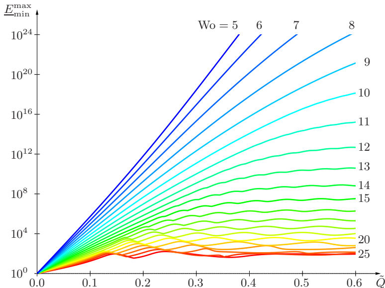
FIGURE 6. Amplitude of intracyclic modulation \underline{E}_{\min}^{\max} at \text{Re} = 10000 and \alpha_1 = 2 for 0 \leq \tilde{Q} \leq 0.6 and 5 \leq \text{Wo} \leq 25 .
