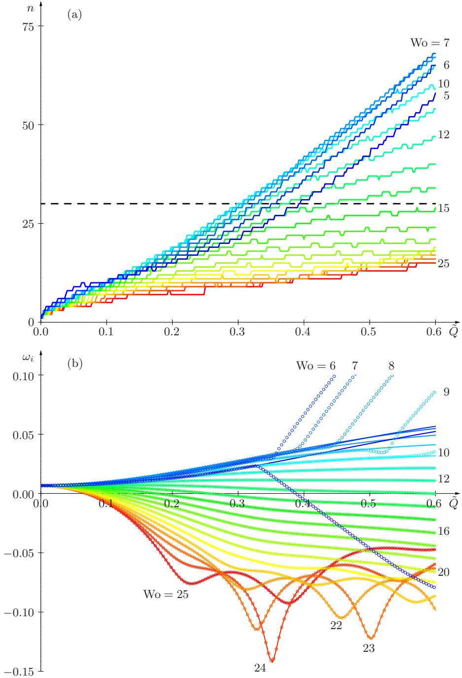
FIGURE 7. Linear dynamics at Re = 10000 and \alpha_1 = 2 for 0 \leq \tilde{Q} \leq 0.6 and 5 \leq Wo \leq 25 . (a) DNS-based estimate of the number of Fourier modes required for a sufficiently resolved Floquet analysis. (b) Comparison of temporal growth rates, computed by linearized DNS (solid lines) and Floquet eigenproblems (symbols) with N_f = 30 . Failure of truncated Floquet analysis (symbols off solid lines in b) largely corresponds to curves above dashed line in (a).
