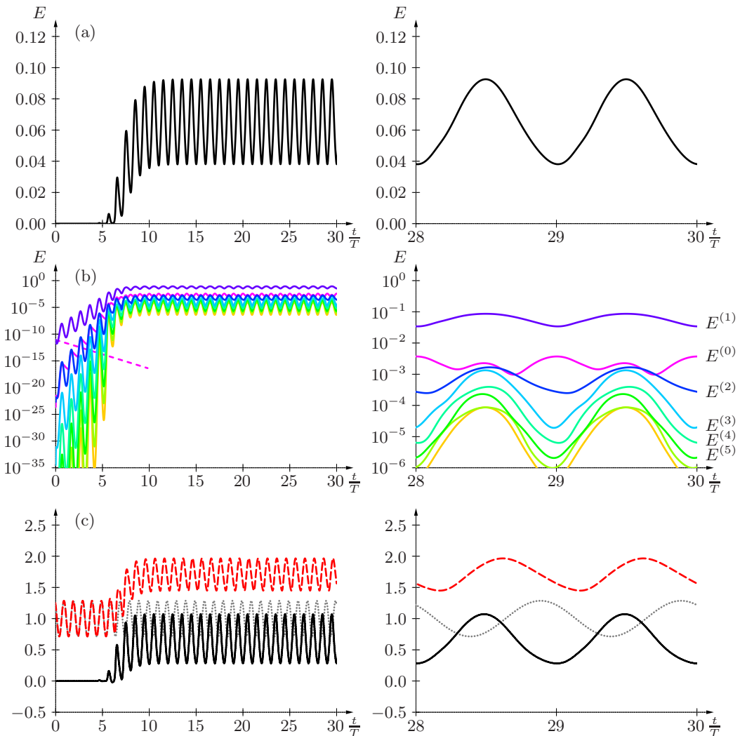
FIGURE 11. “Cruising” nonlinear regime resulting from modulated exponential growth of small-amplitude initial perturbation with \alpha_1 = 2 at \text{Re} = 10000 , \text{Wo} = 10 and \bar{Q} = 0.08 . (a) Total perturbation energy. (b) Energy of each spatial Fourier component. (c) Spatially averaged wall shear stress of perturbation (black solid), total (red dashed) and base (grey dotted) fields relative to steady Poiseuille flow value.
