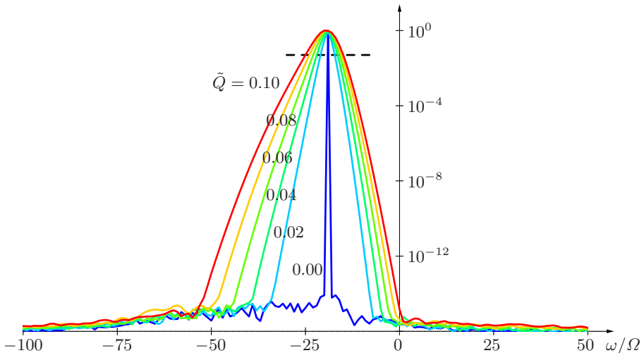
FIGURE 4. Spectra of compensated velocity time series for \tilde{Q} = 0.00, 0.02, \dots, 0.08, 0.10 at \alpha_1 = 2 , Wo = 10 and Re = 10000 . The peak in these spectra near \omega/\Omega = -19 is associated with the dominant frequency -\omega_r of the travelling fluctuations. The width is related to the number of Fourier modes that are required in a Floquet analysis and is seen to rapidly increase with the base-flow pulsating amplitude \tilde{Q} .
