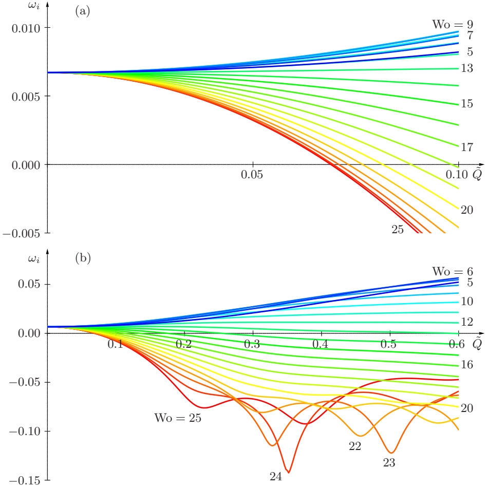
FIGURE 5. Linear temporal growth rate at Re = 10000 and \alpha_1 = 2 for 0 \leq \tilde{Q} \leq 0.6 and Wo = 5, 6, \dots, 25 .
