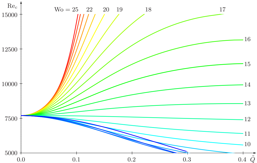
FIGURE 10. Critical Reynolds number for onset of temporal instability as a function of the base-flow pulsation amplitude \tilde{Q} for a range of Womersley numbers: Wo = 5, 6, \dots, 25 .
