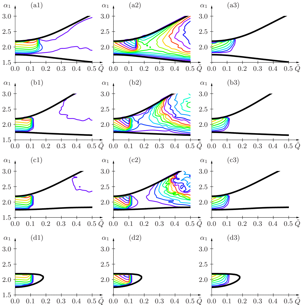
FIGURE 20. Isolines of perturbation energy levels for two-dimensional fully developed nonlinear regimes in (\alpha_1, \tilde{Q}) -plane at \text{Re} = 10000 and (a) \text{Wo} = 6 , (b) \text{Wo} = 10 , (c) \text{Wo} = 12 , (d) \text{Wo} = 15 . Plots (1) represent temporally averaged energy, while (2) and (3) give maximum and minimum values respectively. Color isolines correspond to E = 0.01, 0.02, 0.03, \dots , and the thick black curve represents the neutral boundary.
