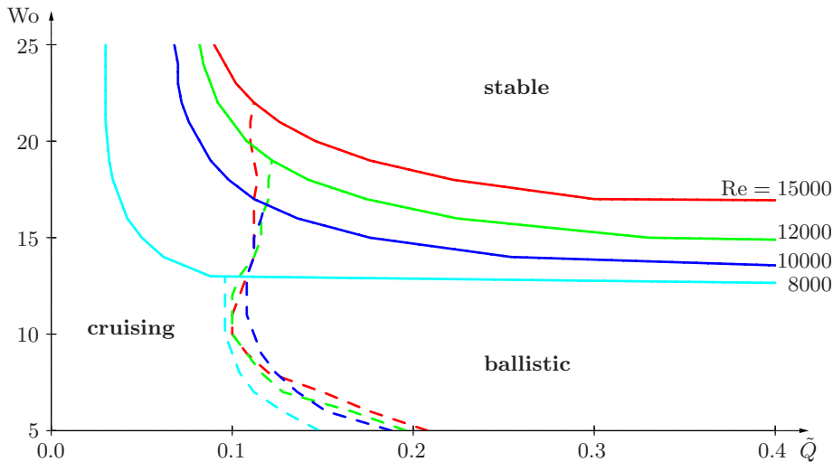
FIGURE 24. Maps in (\tilde{Q}, Wo) -plane indicating nature of the flow dynamics prevailing for a range of Reynolds numbers: Re = 8000, 10000, 12000 and 15000 . Dashed curves correspond to boundary between cruising and ballistic regimes. Above the solid curves the base flows are linearly stable.
