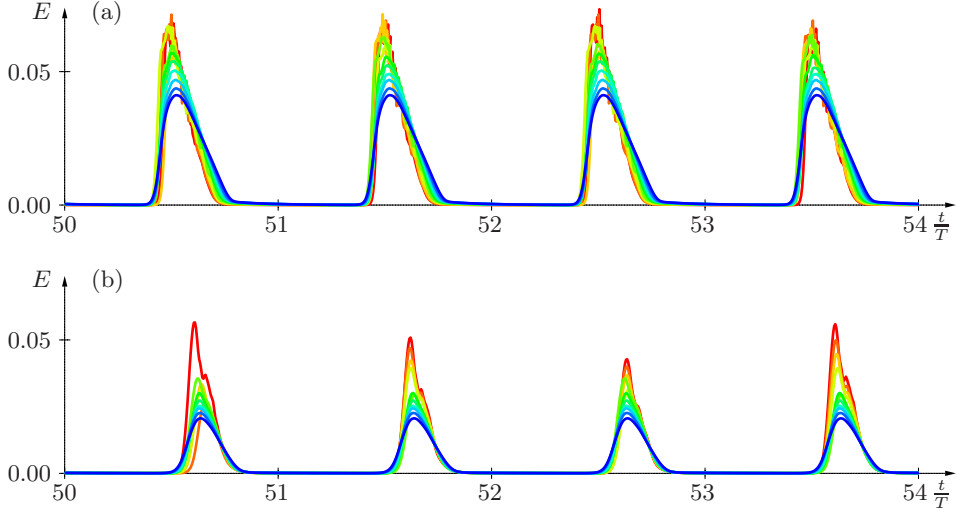
FIGURE 18. Temporal evolution of perturbation energy in fully developed regime at (a) Wo = 7 , (b) Wo = 10 , for \tilde{Q} = 0.20 (blue), 0.22, \dots , 0.38, 0.40 (red) and \alpha_1 = 2 , Re = 10000 . The maximum energy of the nonlinear bursts increases with \tilde{Q} and, at larger values of \tilde{Q} , successive peaks culminate at slightly different levels.
