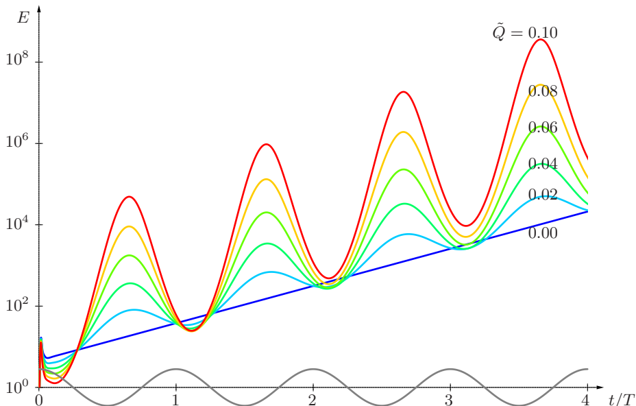
FIGURE 3. Temporal evolution of perturbation energy for \tilde{Q} = 0.00, 0.02, \dots, 0.08, 0.10 at \alpha_1 = 2 , \text{Re} = 10000 and \text{Wo} = 10 (same configurations as figure 2). Intracyclic modulation amplitude rapidly increases with the pulsation amplitude \tilde{Q} , and it is observed that intracyclic growth (resp. decay) approximately coincides with base flow deceleration (resp. acceleration) phases, as indicated by solid sinusoidal line representing Q(t) (not to scale).
