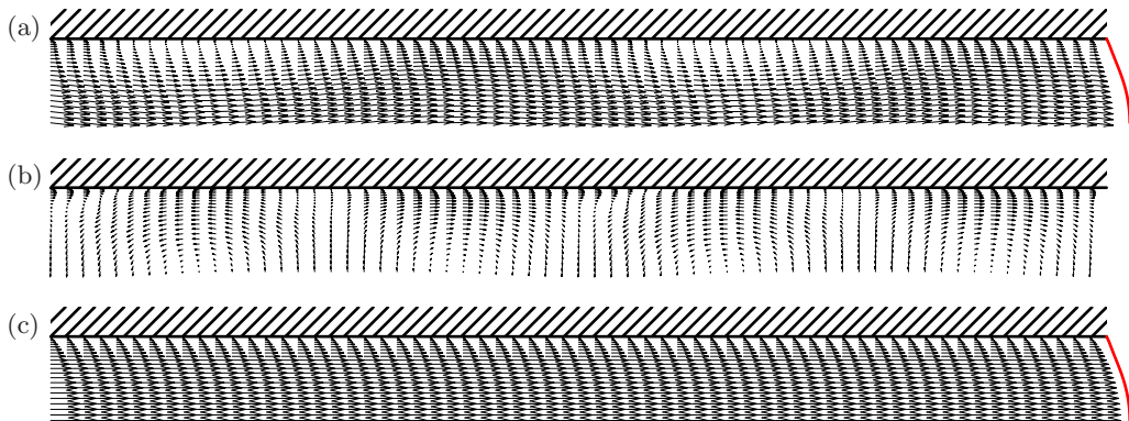
FIGURE 15. Snapshots of velocity fields in ballistic nonlinear regime over two wavelengths with \alpha_1 = 2 at \text{Re} = 10000 , \text{Wo} = 10 and \bar{Q} = 0.2 : (a) total velocity at t/T = 29.6 , (b) perturbation velocity at t/T = 29.6 , (c) total velocity at t/T = 30.0 when the perturbation is negligible. Solid curves to the right of (a) and (c) indicate base-flow profile prevailing at same instant.
