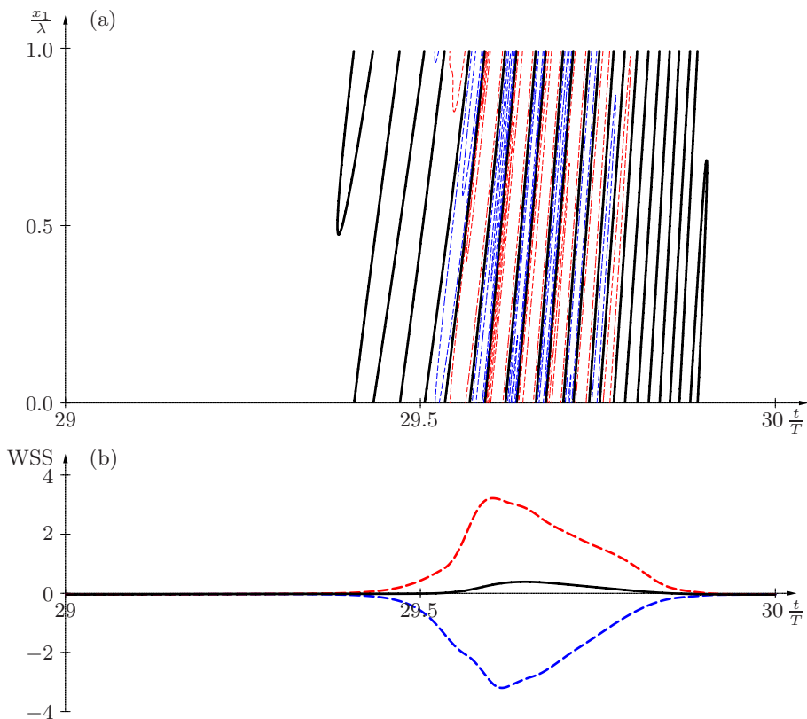
FIGURE 16. (a) Spatio-temporal pattern of the perturbation WSS in ballistic regime over one streamwise wavelength \lambda = 2\pi/\alpha_1 and one pulsation period. WSS values are relative to a steady Poiseuille flow at the same Reynolds number, and thick solid black isoline corresponding to \text{WSS} = 0 separates thin dashed red (resp. blue) isolines corresponding to levels \text{WSS} = 1, 2, 3 (resp. \text{WSS} = -1, -2, -3 ). (b) Instantaneous spatially averaged (solid black), minimum (dashed blue) and maximum (dashed red) values of WSS.
