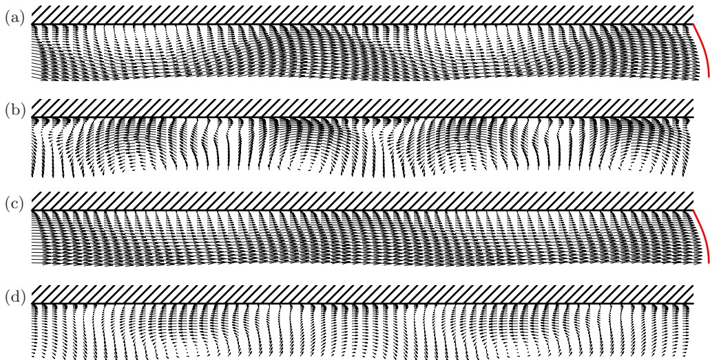
FIGURE 12. Snapshots of velocity fields in cruising nonlinear regime over two wavelengths with \alpha_1 = 2 at \text{Re} = 10000 , \text{Wo} = 10 and \tilde{Q} = 0.08 : (a) total velocity at t/T = 29.5 , (b) perturbation velocity at t/T = 29.5 , (c) total velocity at t/T = 30.0 , (d) perturbation velocity at t/T = 30.0 . Solid curves to the right of (a) and (c) indicate base-flow profile prevailing at same instant.
