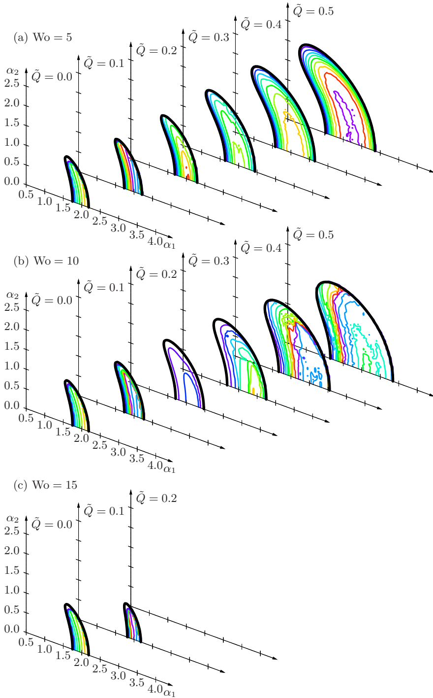
FIGURE 22. Isolines of maximum energy levels for three-dimensional nonlinear solutions in the (\alpha_1, \alpha_2) -wavevector plane for \tilde{Q} = 0.0, 0.1, \dots, 0.5 at (a) Wo = 5 , (b) Wo = 10 , (c) Wo = 15 and Re = 10000 . Color isolines correspond to E = 0.01, 0.02, 0.03, \dots , and the thick black curve represents the neutral boundary.
