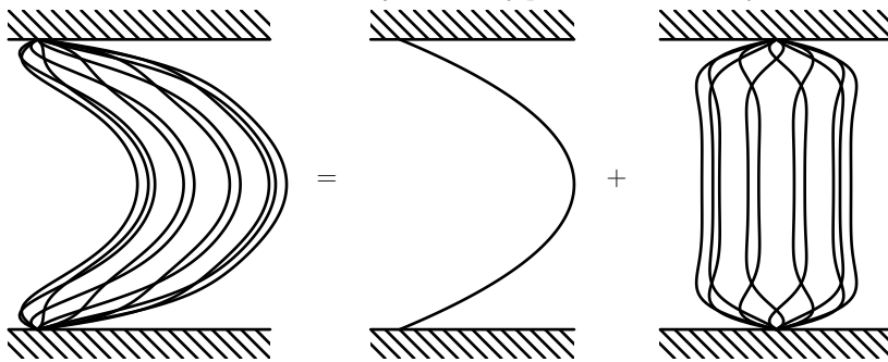
FIGURE 1. Snapshots of typical base flow profile associated with a flowrate of the form Q(t)/Q^{(0)} = 1 + \tilde{Q} \cos \Omega t . In this example, Wo = 10 and \tilde{Q} = 0.6 .
