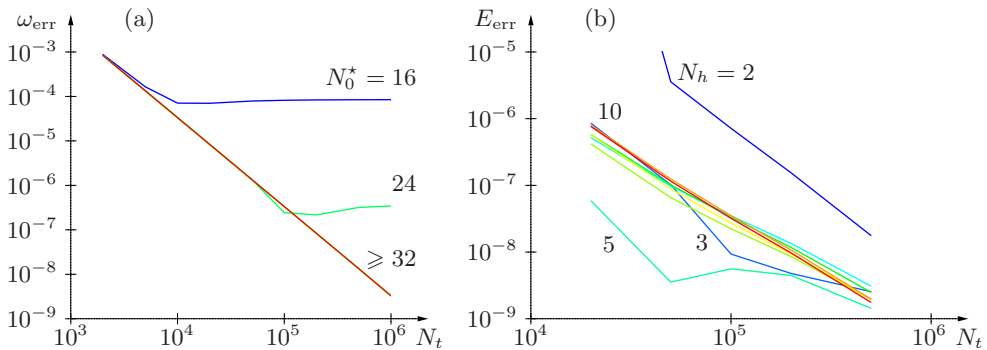
FIGURE 25. (a) Error in \omega computed by linearized DNS with increasing number N_t of time steps per pulsation period and N_0^* = 16, 24, 32, 40, 48 . (b) Error in perturbation energy computed by nonlinear DNS with increasing N_t and N_h = 2 (blue), 3, 4, \dots , 10 (red) at N_0^* = 56 .
