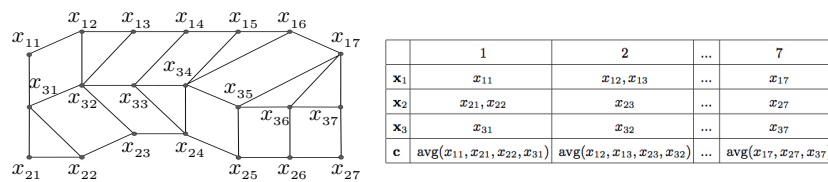
Fig. 3: Centroid estimation based on a reference time series. The DTW is performed between \mathbf{x}_1 , \mathbf{x}_2 and the reference time series \mathbf{x}_3 (left). \mathbf{x}_1 and \mathbf{x}_2 are embedded in the space defined by \mathbf{x}_3 (right) where the centroid is estimated, and 'avg' is the standard mean function.
