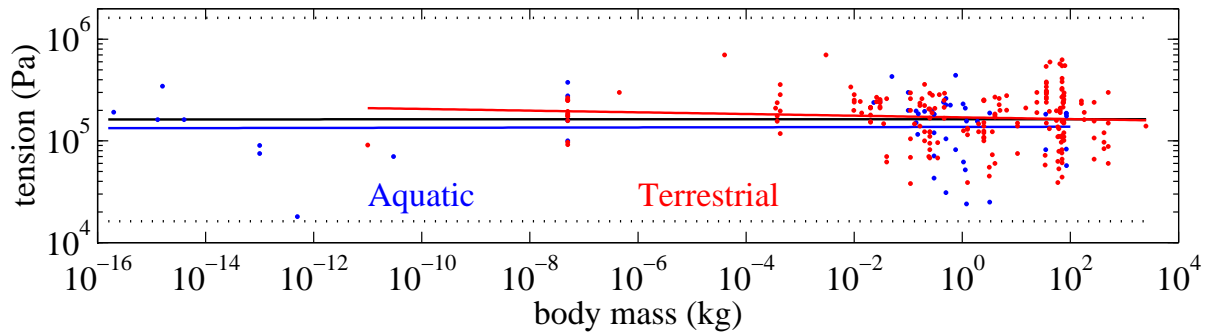
Figure 4. Specific tension used for locomotion versus cell or body mass for terrestrial (in red) and aquatic (in blue) species, and corresponding log-log regression lines, with the regression for all data plotted in black ( \sigma = 10^{5.21} \times M^{0.00} ). The dotted lines are the values smaller and larger by one order of magnitude. For clarity the scale is about twice larger on the tension axis than on the mass axis. (References of the data in Rospars and Meyer-Vernet [22]).
