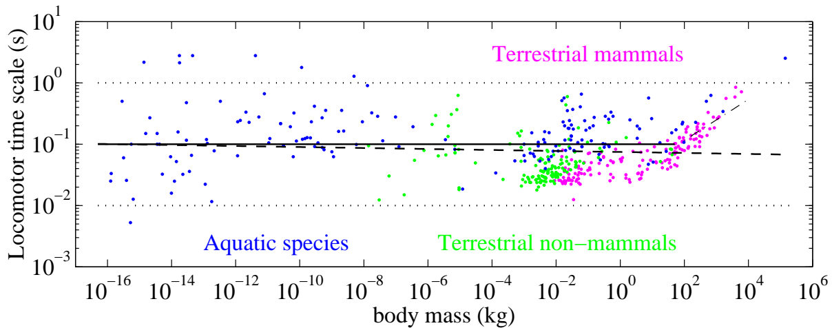
Figure 2. Locomotor time scale as a function of body mass for terrestrial mammals (in magenta) and non-mammals (in green), and aquatic species (in blue) from the references cited in subsection 2.3. The dashed line \tau = 10^{-1.127} \times M^{-0.008} is the regression of \log_{10}\tau versus \log_{10}M for the whole data set. The solid line (with values smaller and larger by one order of magnitude dotted) is from (6), estimated in section 3; the limit for large masses estimated in subsection 3.4 is shown dash-dotted. For clarity the scale is twice larger on the speed axis than on the mass axis.
