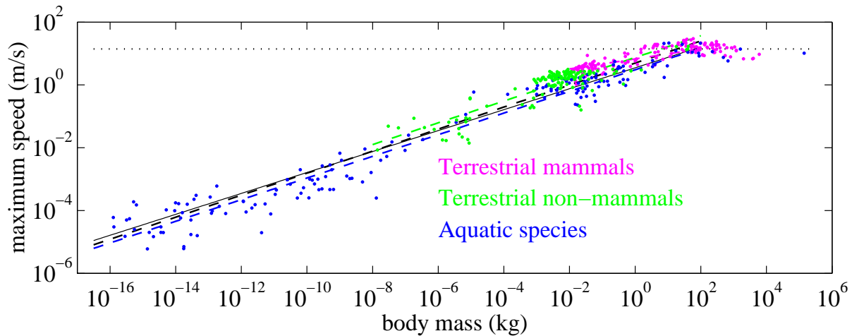
Figure 1. Maximum speed versus body mass for terrestrial mammals (in magenta) and non-mammals (in green), and aquatic species (in blue) from the references cited. The corresponding regression lines are shown (dashed) in similar colors, and the regression line for all data is shown in (dashed) black. Maximum running and swimming speed (black solid line, equation (7)) and upper limit at large masses (dotted) are also shown as estimated in section 3.
