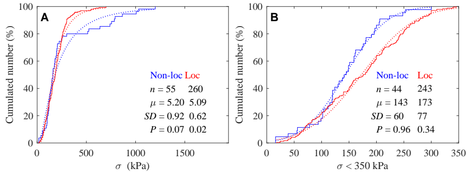
Figure 3. Empirical cumulative distribution functions (CDFs) of the specific tension \sigma used for locomotion (red) and other functions (blue) in aquatic and terrestrial species. Panel A shows empirical CDFs of all \sigma values (solid) fitted to lognormal CDFs of mean \mu and SD indicated (dotted). Panel B shows empirical CDFs of values \sigma < 3.5 \times 10^5 Pa fitted to Gaussians (dotted) of mean and SD indicated. CDFs of locomotors and non-locomotors are not significantly different at level 5% ( P = 0.13 ) in A and significantly different ( P = 0.01 ) in B. All comparisons based on Kolmogorov-Smirnov tests. (References of the data in Rospars and Meyer-Vernet [22]).
