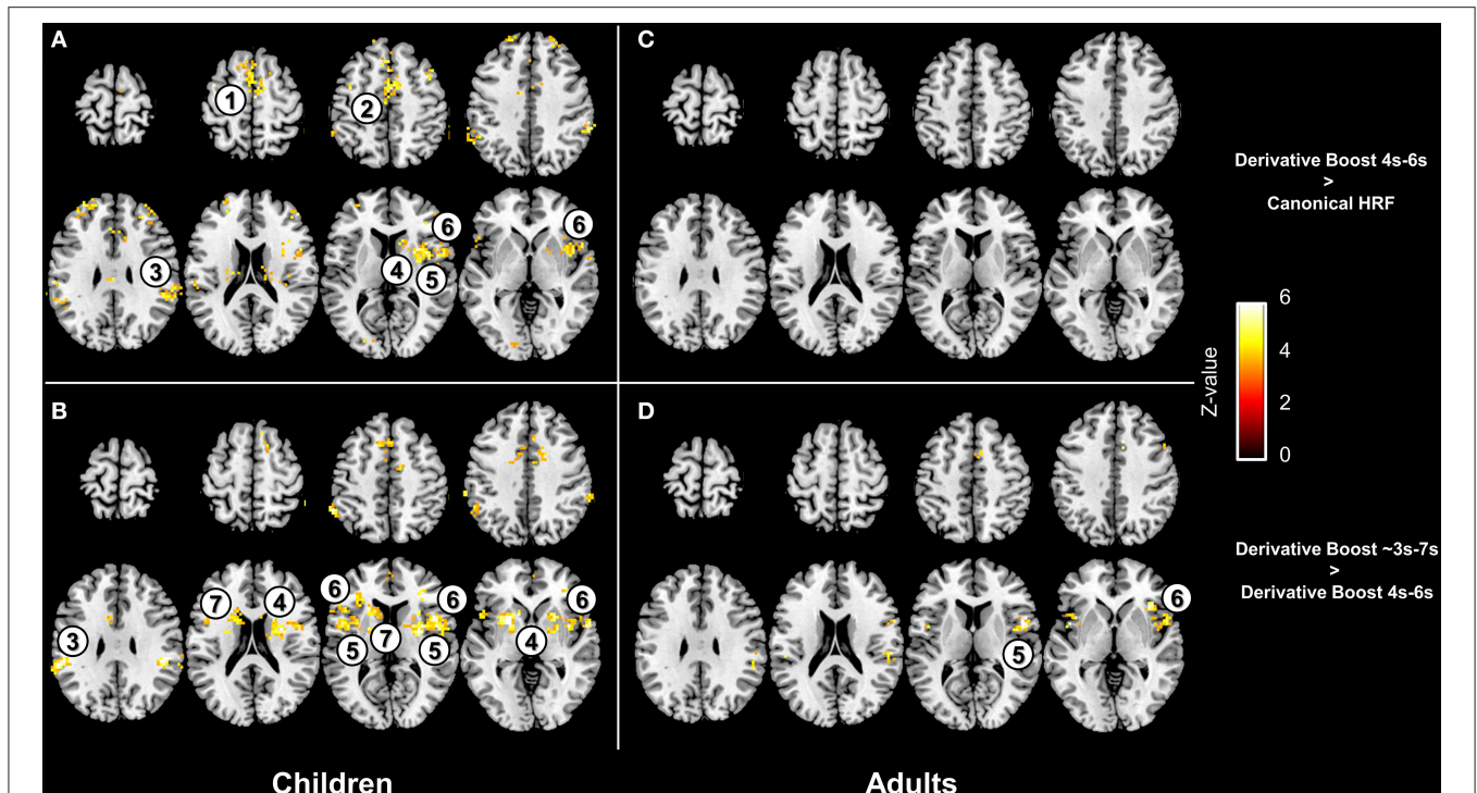
FIGURE 4 | Effect of the derivative boost on amplitude estimates in the 100 Hz proprioceptive condition. Panel (A,C) display voxels where amplitude estimate is increased while using the derivative boost constrained between 4 and 6 s (as compared with the model including the canonical HRF alone) in children and adults. Panel (B,D) illustrate additional increase in amplitude estimates while using the full derivative boost compared to that constrained between 4 and 6 s, in children and adults. Maps are thresholded at a voxel-wise threshold of p < 0.001 uncorrected and a cluster extend threshold of p < 0.05 FWE-corrected. Numbers refer to main regions in which amplitude estimate was increased; 1, supplementary motor area; 2, anterior cingulate cortex; 3, inferior parietal lobule; 4, putamen; 5, anterior insula; 6, inferior frontal gyrus; 7, caudate.
