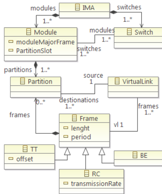
Fig. 6. The Metamodel of IMA.
