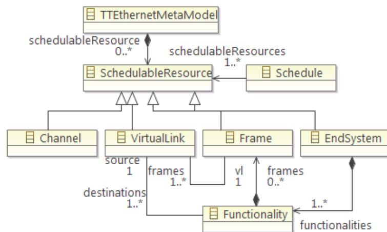
Fig. 3. Schedulable resources.
