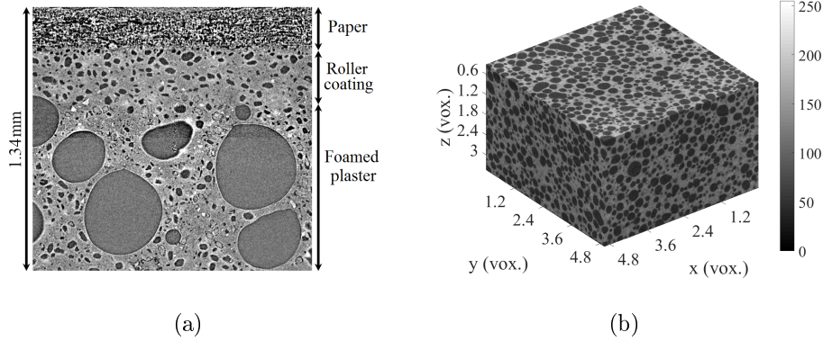
Figure 1: (a) Tomographic section showing the microstructure observed at a resolution of 1.4 \mu\text{m} of the studied plaster whose porosity is of the order of 75 %. The size of the section is 1.34 \times 1.4 \text{ mm}^2 . (b) 3D rendering of the microstructure of the core material studied herein and observed at a resolution of 12 \mu\text{m} . The size of the volume is 4.8 \times 4.8 \times 3.2 \text{ mm}^3
