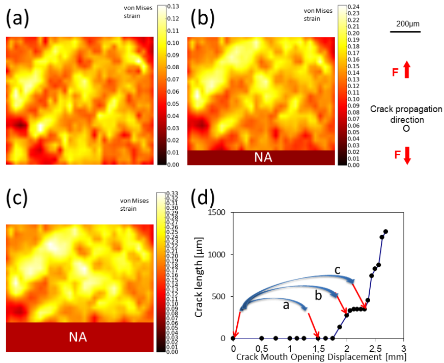
Figure 7: 2D sections of cumulated equivalent von Mises strain fields. (a) Direct correlation from CMOD = 0.0 mm to CMOD = 1.5 mm. (b) One cumulation from CMOD = 0.0 mm to CMOD = 2.0 mm. (c) Two cumulations from CMOD = 0.0 mm to CMOD = 2.313 mm (the coordinate system is shown in its initial state)
