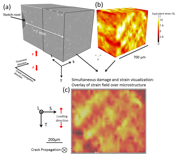
Figure 5: (a) 3D rendering of the initial microstructure and the ROI. (b) 3D rendering of the equivalent strain field in the extracted volume when \text{CMOD} = 1.5 \text{ mm} . (c) 2D overlay of strain field over the initial microstructure
