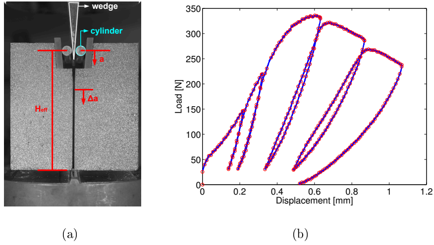
Figure 1: (a) Picture showing the geometry of WST. The surface has been prepared for DIC purposes. The wedge and cylinders used for the loading are highlighted. H_{eff} corresponds to the loaded height, a is the crack length considering the loading point as a = 0 , and \Delta a is the measured propagation increment. (b) Loading curves with blue dots showing machine acquisition and red circles interpolated points for each image taken during the test
