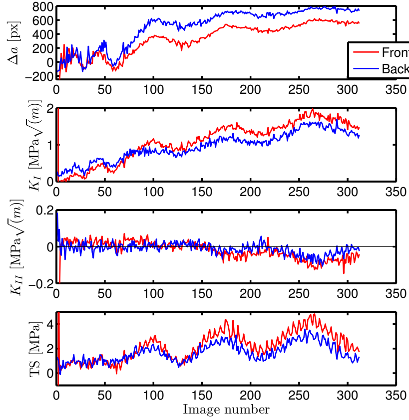
Figure 8: Results for the front and back faces with p_f = 8 . The measured crack length, SIFs and the T-stress are shown
