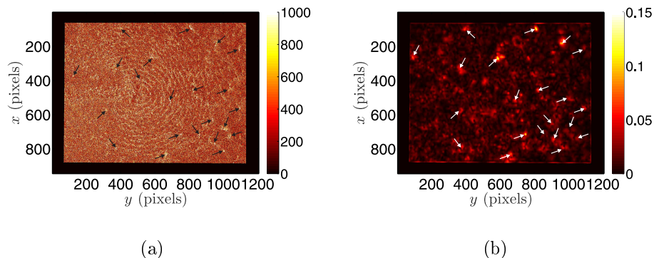
Figure 10: Mesoscale (a) correlation (in gray level) and (b) mechanical residual maps corresponding to maximum load level ( i.e. , F_1 = F_2 = 40 kN) for the first cycle of EBE-1 experiment. The arrows indicate the detected cracks. 1 pixel \leftrightarrow 6.7 \mu\text{m}
