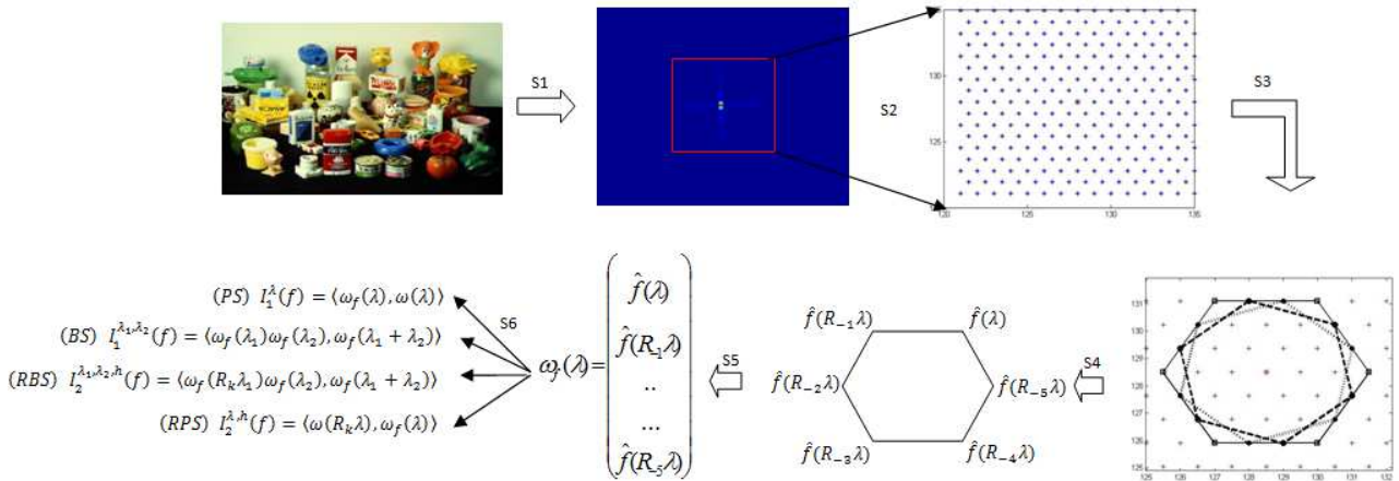
Fig. 1 Steps of computing the invariant descriptors. (S1) computation of the shifted FFT of the the image f , (S2) generation of the hexagonal grid, (S3) extraction of different hexagons, (S4) evaluation of the FFT of f on each extracted hexagon, (S5) generation of the vector \omega_f(\lambda) and (S6) computation of the four invariants
