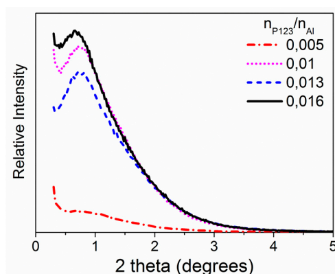
Figure 1. Small angle XRD for P123/Al molar ratios ranging from 0.005 to 0.016.
