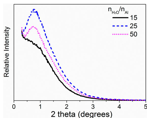
Figure 5. Impact of water content on small angle XRD.
