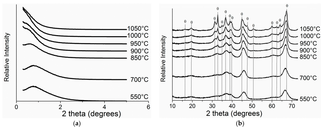
Figure 7. Impact of the thermal treatment by (a) small angle XRD; (b) wide angle XRD.
