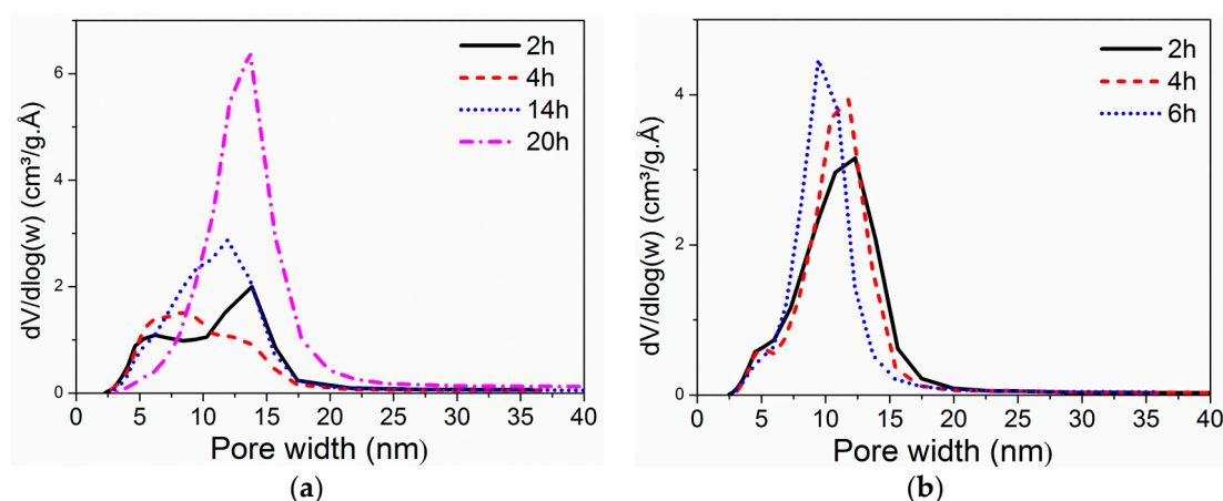
Figure 4. Pore size distribution from N 2 isotherms, impact of peptization at (a) 85 °C and (b) 100 °C.
