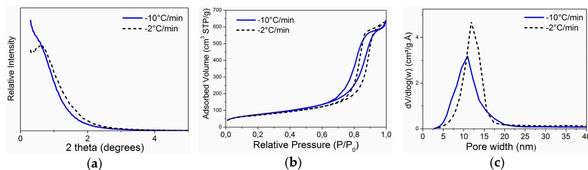
Figure 6. Impact of cooling speed on (a) XRD; (b) N 2 isotherm and (c) pore size distribution.
