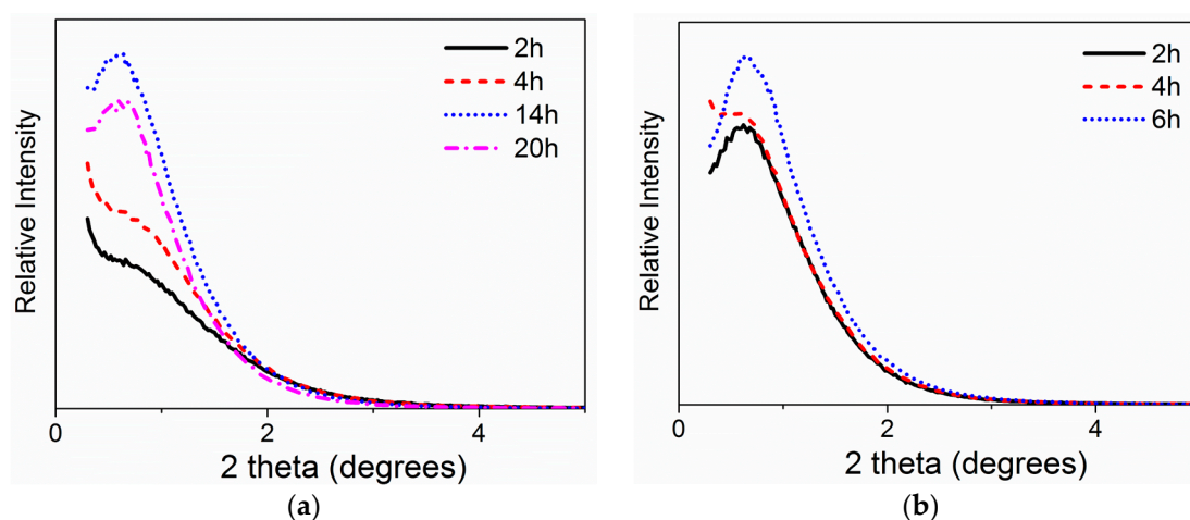
Figure 3. Impact of peptization duration on small angle XRD at (a) 85 °C and (b) 100 °C.
