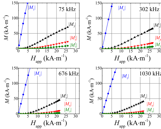
FIG. 1. The magnitude of different harmonics (1 st , 3 rd , 5 th and 7 th ) for different applied magnetic field intensities at each frequency measured at 25 °C. The high order harmonics start to rise above 5 \text{ kA}\cdot\text{m}^{-1} .
