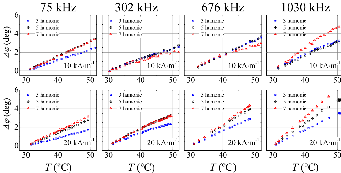
FIG. 2. Variations of harmonic phases \Delta\varphi (relative to the phase at 30 °C) with temperature.
