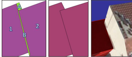
Fig. 15. Elongated polygons A and B are detected (left) and are respectively merged to footprints 1 and 2 (middle) in order to propose two distinct footprints that will give a visually satisfying 3D geometry (right).
