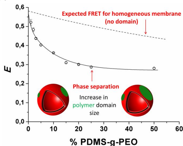
Figure 3: FRET efficiency versus content (mol %) PDMS- g -(PEO) 2 . Solid line is a guide to the eyes.
