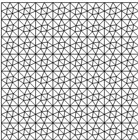
Figure 1: Co-volumes centred on faces.
