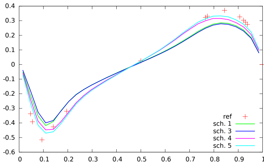
Figure 3: Lid driven cavity, vertical velocity profile along the line y = 0.5
