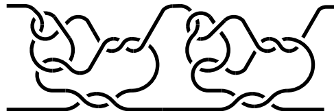
FIGURE 2. The key tangle M_1 = T_{20} .
