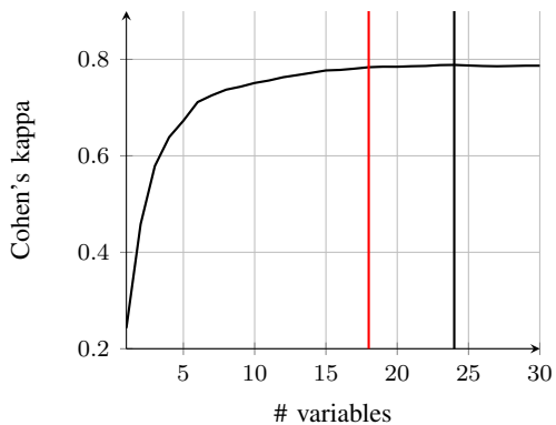
Fig. 5. Criterion evolution (kappa) in function of the number of selected variables for first trial with Aisa dataset with 500 samples by class. Red vertical line is the retained number of variables and black vertical line is the maximum of the criterion.
