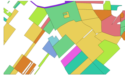
Fig. 3. Aisa dataset: (a) colored composition of the image (R: 634nm, G: 519nm, B: 477nm), (b) ground-truth.
