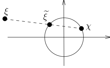
Fig. 2.1. Definition of the additional variable \tilde{\xi} for the case p \in (1, 2) .
