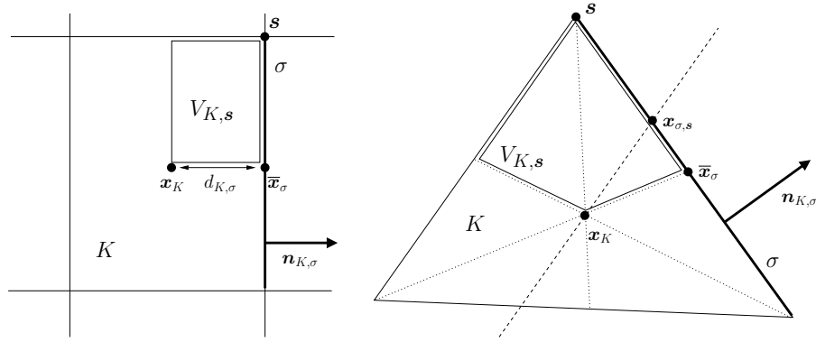
Fig. 11.1. Notations for MPFA-O schemes defined on Cartesian (left) and simplicial (right) meshes.
