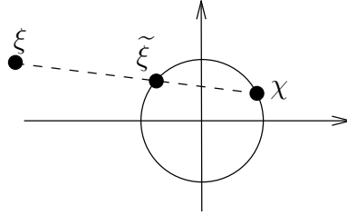
Fig. 3.1. Illustration of the proof of (3.85) in the case p \in (1, 2) .
