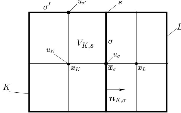
Fig. 1.2. Notation for a rectangular mesh.
