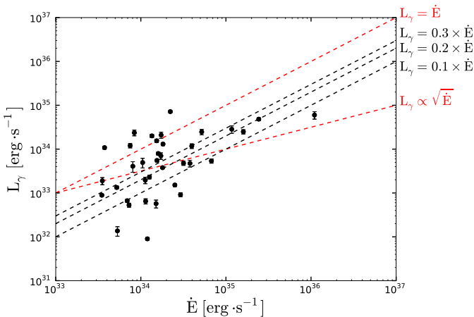
Fig. 3. Observed \gamma -ray luminosity L_\gamma versus spin down power \dot{E} for the 36 Fermi -LAT MSPs used in this study. The dashed lines indicate empirical laws used to predict the \gamma -ray luminosity of individual MSPs (see text).
