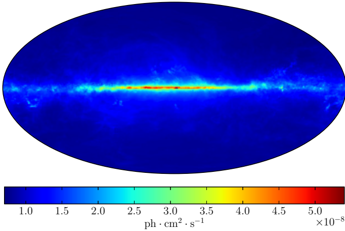
Fig. 4. Sensitivity map of the Fermi -LAT for detection of IFGL point sources, which are given in Galactic coordinates and Aitoff projection (Abdo et al. 2010c).
