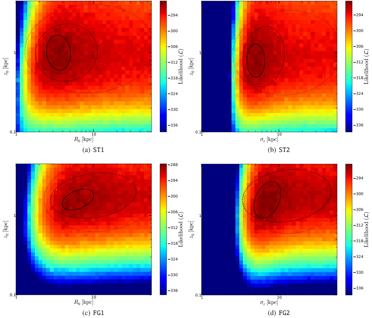
Fig. 5. Log-likelihood as a function of radial scale length ( R_0 or \sigma_\tau ) and vertical scale height ( z_0 ) for four MSP population models (see text). Contours show the 1, 2, and 3\sigma confidence ellipses that have been computed from the log-likelihood maps (colours). All maps show the same dynamic range in log-likelihood.
