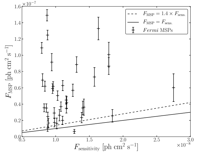
Fig. 7. Fermi -LAT MSPs flux above 100 MeV ( F_{\text{MSP}} ) against the sensitivity ( F_{\text{sensitivity}} ). Solid and dashed lines show F_{\text{MSP}} = F_{\text{sensitivity}} and F_{\text{MSP}} = 1.4 \times F_{\text{sensitivity}} respectively.
