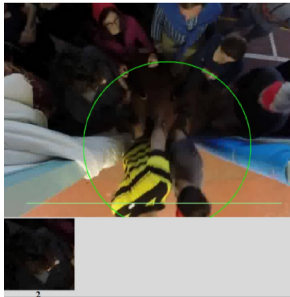
Figure 2 One randomly selected video frame, with the exit zone marked in light green. A home-made Python routine allows us to click on the pedestrians when they enter the zone and deselect them when they exit.
