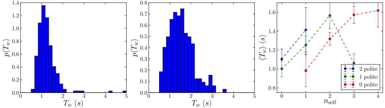
Figure 7 Dwell times T_w in the exit zone in evacuations with hurried walkers. Normalised histograms of T_w for c_s^* = 0\% (hurried) (left) and c_s^* = 100\% (hurried) (middle). The right panel shows the average dwell time for selfish, hurried pedestrians as a function of the number n_{\text{self}} of selfish participants in the zone, for distinct numbers of polite participants. The error bars are 95% confidence intervals. Note that these averages were computed from subsamples of n \approx 20 - 200 data points, except in the cases of 0 polite agent and 1 selfish one ( n = 11 ) and 1 polite agent and 3 selfish ones ( n = 6 ).
