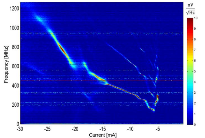
Fig. 3. Dependence of the microwave frequency on DC current for a SL STO with 110 nm nano-contact diameter. The current was varied from -30 mA to 0 mA at zero applied magnetic field.
