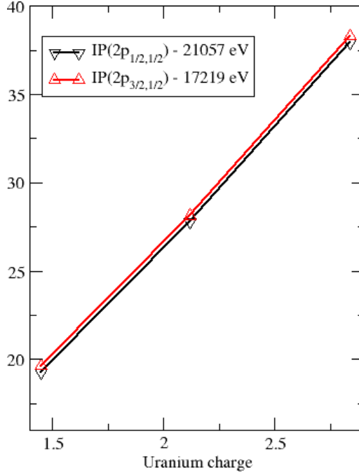
Figure 1: Shifted \Delta HF uranium 2p ionization energies of the title species (in eV) as a function of the uranium charge (in a.u.) from projection analysis.
