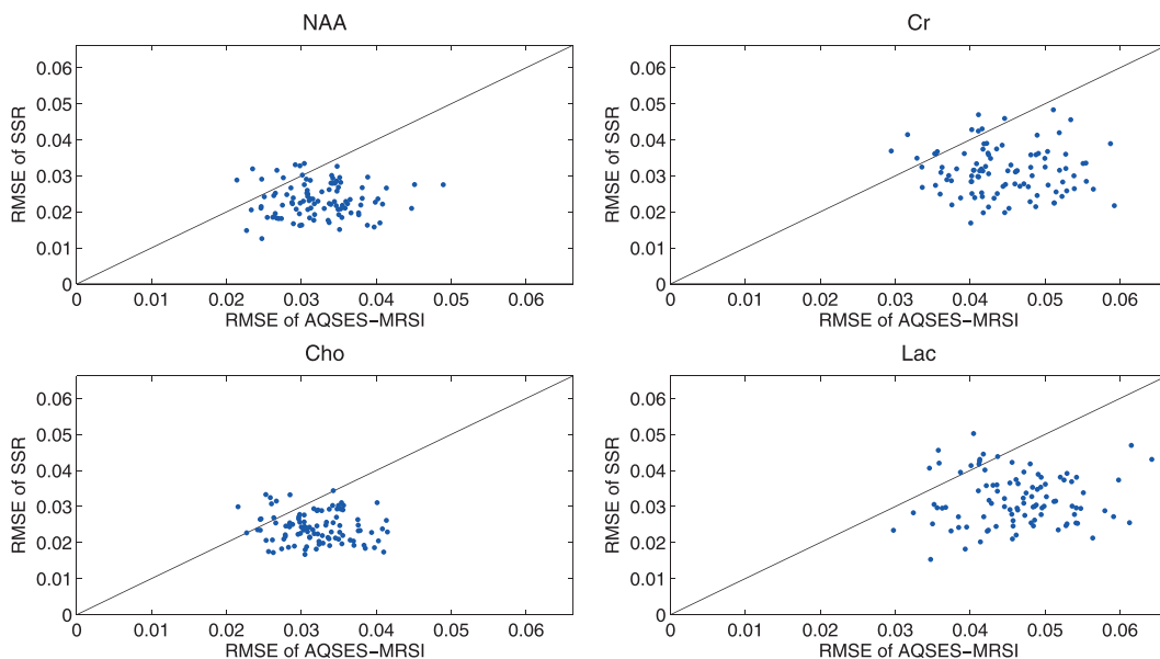
Figure 6. RMSE_{k,r} of the estimated metabolite amplitudes obtained with the proposed method (SSR) and with AQSES-MRSI for 50 synthetic MRSI data sets of size 10 \times 10 at SNR = 4.5. Each point corresponds to one voxel of the MRSI grid.
