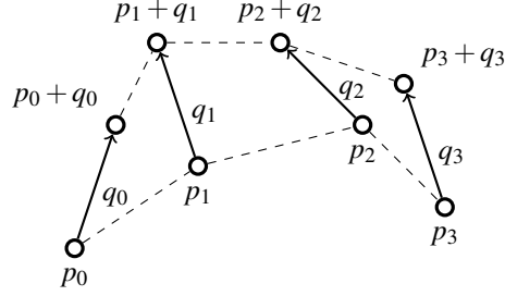
Figure 5: Displacement of a polygon.
