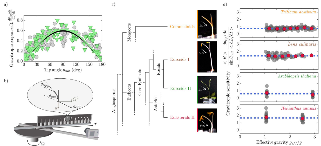
Figure 3. Gravitropic response is independent of effective gravity. (a) Normalized gravitropic response of wheat coleoptiles as a function of inclination angle \theta_{mit} at 1g (grey circles) and 2.5g (green triangles). Black and green curves are the respective fitted sine functions. (b) Sketch of the experimental setup. Plants in a chamber (60 cm \times 16 cm \times 3 cm) are rotated at an angular velocity \Omega about a vertical axis. Centrifugation creates an effective gravity g_{eff} . \theta_{mit} and \theta_{tip} are the initial angle of the plant and the angle of the tip relative to the direction of g_{eff} . (c) Simplified phylogenetic tree (adapted from the Angiosperm Group Phylogeny III classification, http://www.mobot.org/mobot/research/apweb/ ) showing relationships between the four species studied (from top to bottom): Triticum aestivum , wheat coleoptile; Lens culinaris , lentil stem; Arabidopsis thaliana , Arabidopsis inflorescence stem; Helianthus annuus , sunflower hypocotyl. (d) Gravitropic sensitivity \beta plotted as a function of the gravity intensity for the four species in (c). As the elongation rate was independent of g_{eff} (Supplementary Fig. S2), a mean elongation rate was used to compute \beta . Means of values in bins of equal ranges in gravity intensity are shown (red circles) with the mean of the whole dataset (dashed blue lines).
