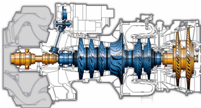
Fig. 1. Helicopter turboshaft RTM322 (Turbomeca–Rolls Royce)—An example of turbomachine.
