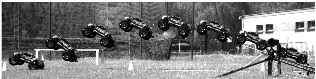
Figure 2: Sequential view of an actual in-field jump with RobCat. The change in RobCat's pitch attitude at the end of the ballistic phase was induced by an acceleration of its wheels by the pilot.
