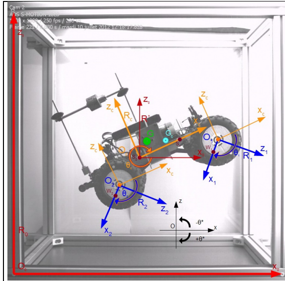
Figure 3: RobCat at rest in the test bench. Reference frames and variables used in the model are indicated.
