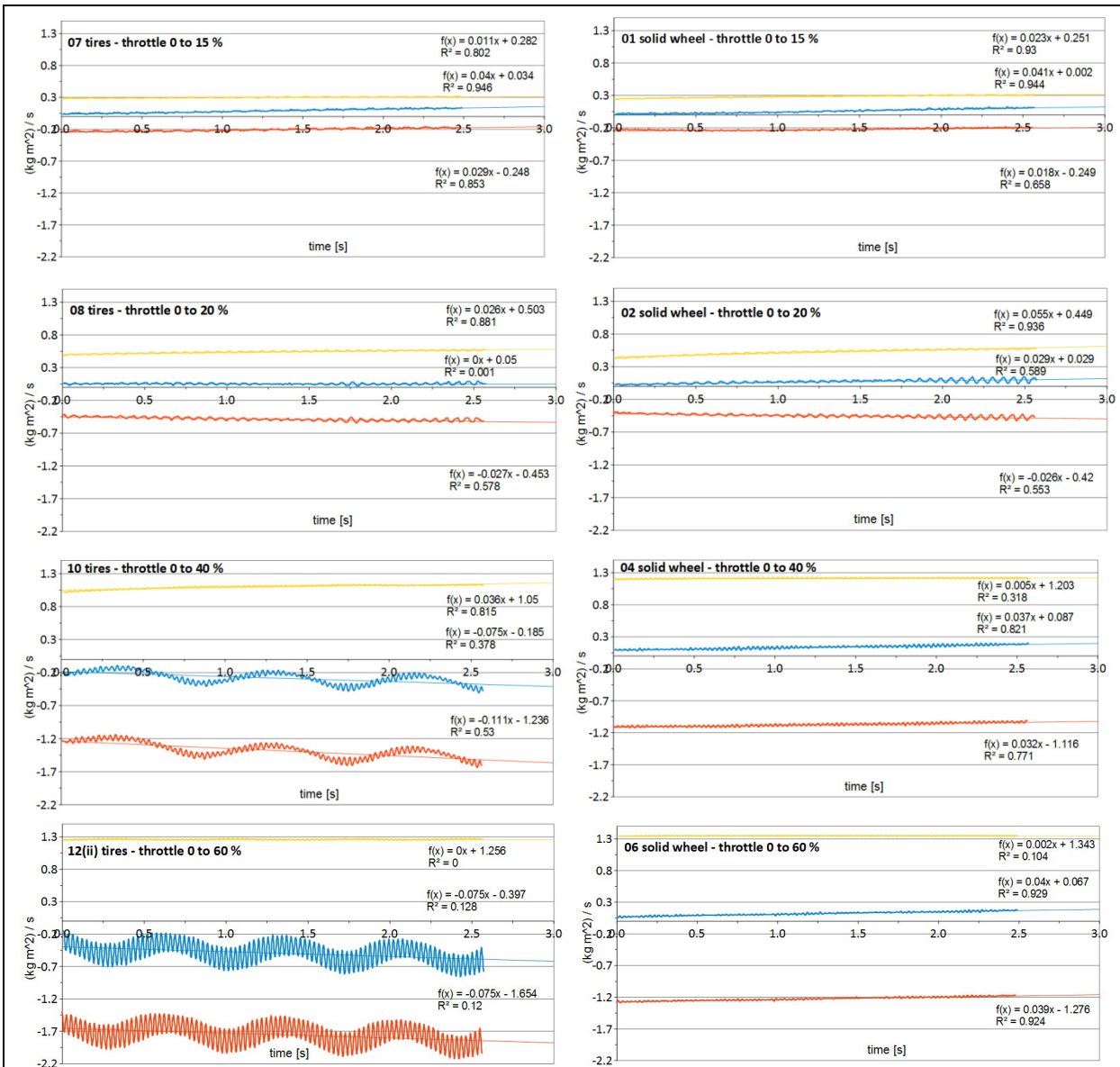
Figure 4: Total (blue) and partial angular momenta of RobCat's system (red) and wheels (yellow) equipped with rubber tyres (left column) or solid wheels (right column) during selected trials performed on the test bench at 15% (first line), 20% (second line), 40% (third line) and 60% (last line) of the engine power.
