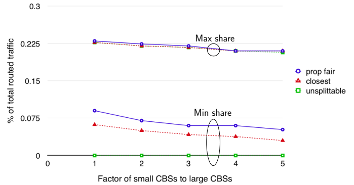
Fig. 4. Minimum and maximum load share of a small (2nd tier) CBS depending on the ratio of small CBS number over large CBS number.
