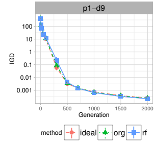
Fig. 5. GD and IGD in DTLZ3.
