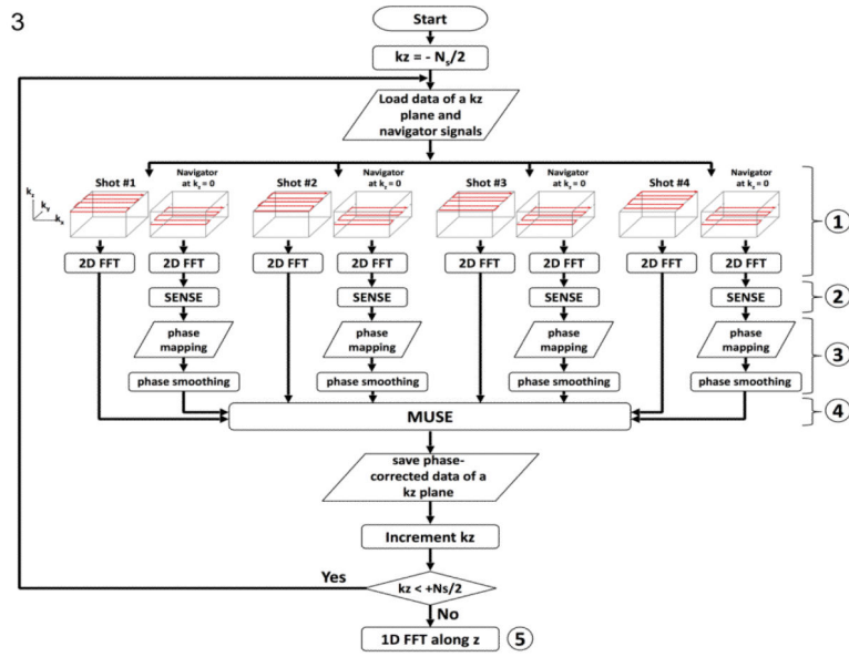
Figure 3. The flow chart of reconstructing 3D interleaved DW-EPI data with 3D MUSE algorithm.
