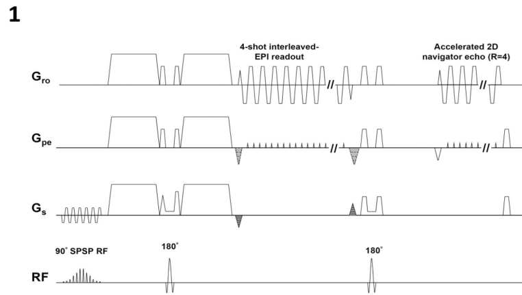
Figure 1. A slab-selected 3D interleaved EPI pulse sequence that acquires diffusion weighted signals and accelerated navigator signals.
