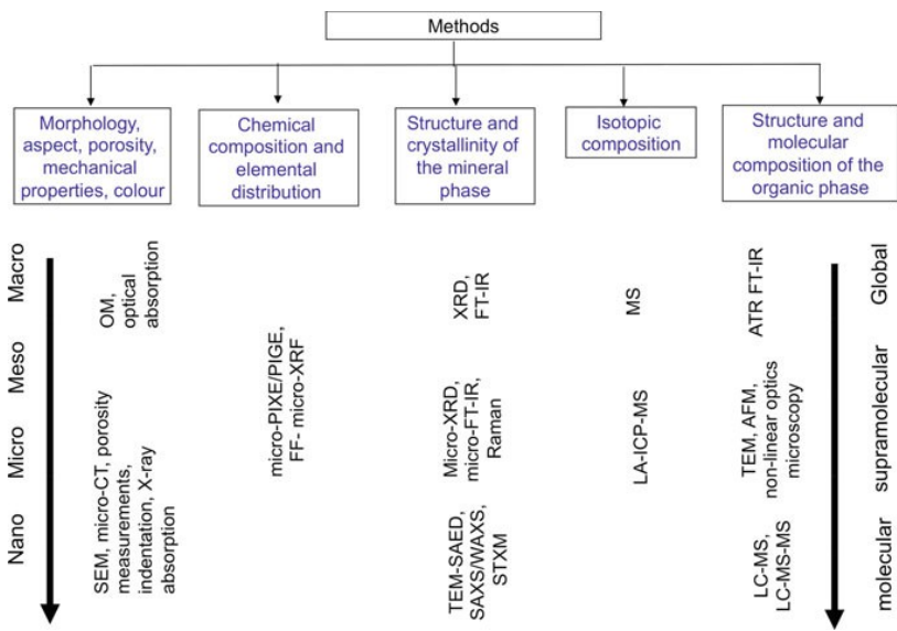
Figure 7 Overview of the generally used analytical techniques for obtaining complementary information on the structure and composition at different length scales of biominerals
