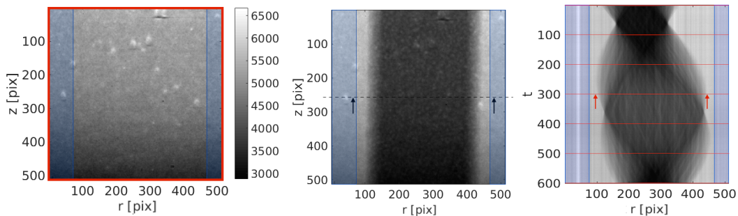
Fig. 1. (a) Flat-field captured between t = 300 and t = 301 (the spatial inhomogeneity of the flat-field is quite pronounced with bright spots and an overall intensity gradient). (b) Raw projection at t = 300 , where the two regions \Omega_l and \Omega_r are the blue shaded rectangles, and the central darker region is caused by the specimen absorption. (c) In a space-time ( r-t ) diagram (sliced at a given height, z = 256 pixels) full flat-fields, f , are shown as red lines to indicate that they cover the entire detector but are captured only at some interruptions of the scan and sinogram borders \Omega_l and \Omega_r , shown in blue to highlight that they are available at all times but only over a limited portion of the detector
