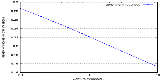
Fig. IV.9. Density of successful transmission versus the capture threshold T ( \lambda=1, \mu = 10, T = 1 ). Linear network (1 D)
