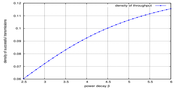
Fig. IV.10. Density of successful transmissions versus the decay factor \beta for 2D networks ( \lambda=1, \mu = 10, T = 1 ).
