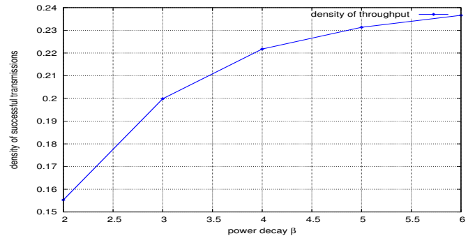
Fig. IV.11. Density of successful transmissions versus the decay factor \beta ( \lambda=1, \mu = 10, T = 1 ). Linear network (1 D)
