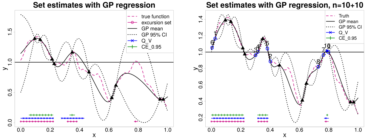
(a) Initial DoE: maximin LHS, n = 10 . (b) Adaptive DoE: strategy T2 , 10 new points.
