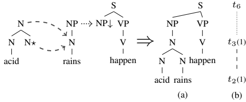
Figure 1: Tree rewriting in TAG resulting in a derived tree (a), and a derivation tree (b).
