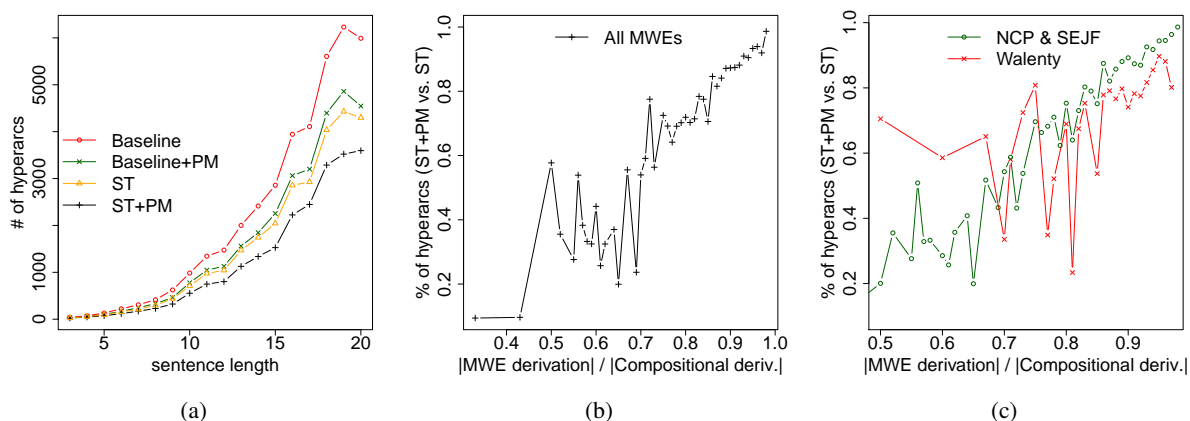
Figure 4: (a) Average number of hyperarcs explored depending on the parsing strategy (for clarity using only sentence of length < 20 ), (b) Average % of hyperarcs explored with the PM+ST strategy, using the ST strategy as a reference, and (c) Average % of hyperarcs explored depending on the type of MWEs.
