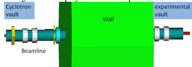
Figure 2: Layout of the G4Beamline simulation.
