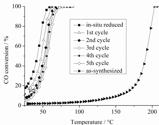
Figure 1. Light-off curves for CO oxidation of the as-prepared, in-situ reduced and cycled 2.5 wt-%Pt/CeO 2 catalysts.
