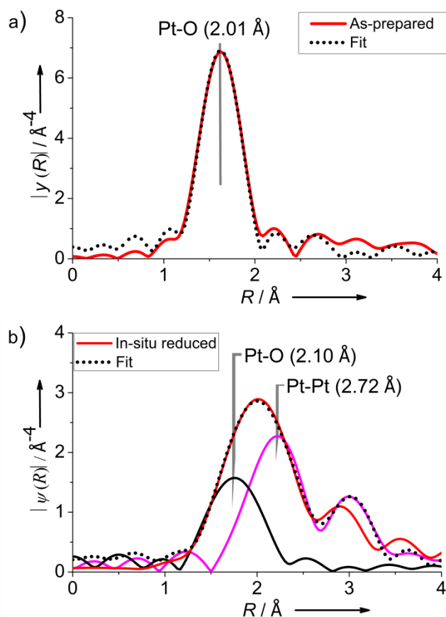
Figure 3. FT of EXAFS spectra of a) as-prepared and b) in-situ reduced 2.5 wt-% Pt/CeO 2 catalysts together with the best fits and the contributions of Pt-O, Pt-Pt.
