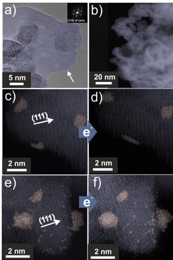
Figure 2. (S)TEM images of Pt/CeO 2 catalysts. a) HRTEM image of Pt nanoparticles supported on ceria. The arrow in a) points to a Pt nanoparticle spread on the surface of ceria. The inset shows the power spectrum of the ceria support. b) to d) HAADF-STEM images of Pt/CeO 2 catalyst after reductive activation in H 2 at different magnifications. c) Atomic resolution HAADF-STEM image and (d) corresponding HAADF-STEM image after exposure to the electron beam for 37 s. e) HAADF-STEM image after CO oxidation and f) HAADF-STEM image of the same position after exposure to the electron beam for 302 s. The ceria support is highlighted in blue, whereas the Pt nanoparticles are depicted in red. The original images are given in the supporting information, Figure S2.
