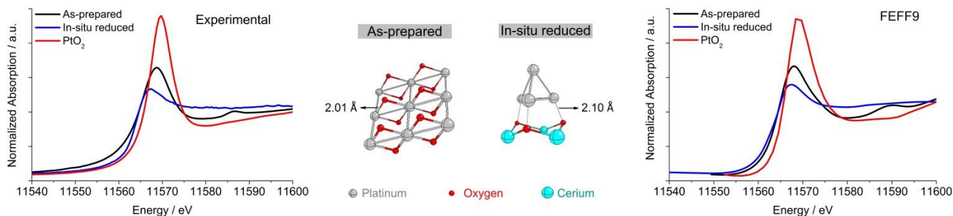
Figure 4. Experimental PtL 3 -edge XANES patterns of the as-prepared as well as in-situ reduced 2.5wt-%/CeO 2 (left side) and the simulated ones with FEFF9 code (right side) along with the proposed model structures (middle panel).
