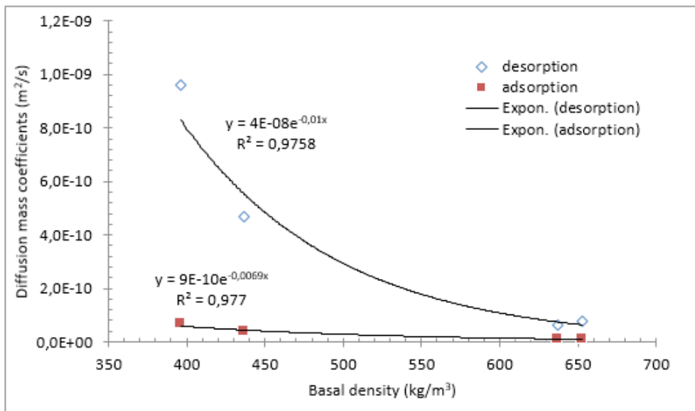
Figure 19. Evolution of mass coefficient diffusion with the basal density.
