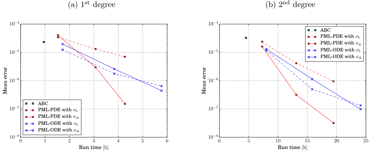
Figure 6: Mean error over the period [250 ms, 500 ms] as a function of the runtime.
