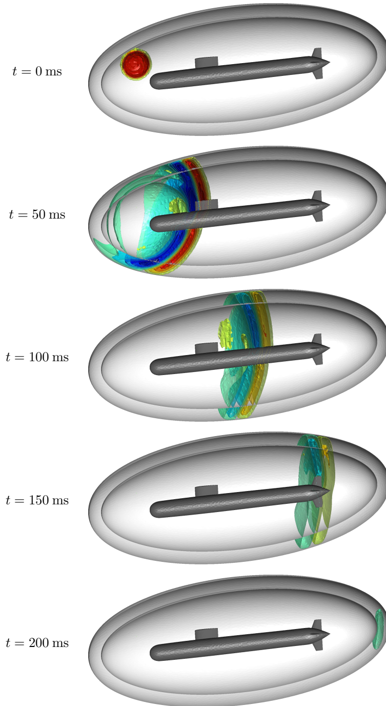
Figure 7: Snapshot of the solution of the three-dimensional benchmark at different instants. Colored surfaces are iso-surfaces of p(\mathbf{x}, t) . The inner and outer white surfaces correspond to the interior and exterior boundaries of the PML, respectively
