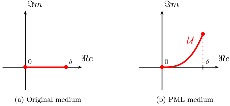
Figure 2: Complex coordinate stretch of the radial coordinate \xi_1 .
