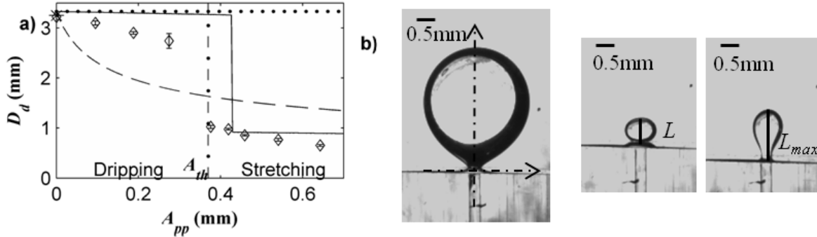
Figure 2: (a) Drop diameter D_d depending on the peak-to-peak capillary amplitude A_{pp} for f = 100 Hz, D_p = 0.32 mm, q = 4.3 \mu\text{L.s}^{-1} : ( \diamond ) measurements, measured amplitude threshold (dash-dotted line), (*) estimates from eq. (1), estimates from the balance F_b = F_Y^{max} (dotted line), estimates from the balance F_b + F_{exc}^{peak} = F_Y^{max} (dashed line), estimates from eq. (9) (solid line). (b) Drop image just before detachment in dripping mode (left, A_{pp} = 0.095 mm), in stretching mode (centre and right, A_{pp} = 0.419 mm).
