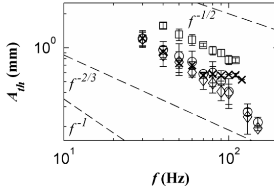
Figure 3: Threshold amplitude depending on the forcing frequency: ( \square ) D_p = 0.11 mm, q = 2.2 \mu\text{L.s}^{-1} , ( \diamond ) D_p = 0.32 mm, q = 6.5 \mu\text{L.s}^{-1} , ( \circ ) D_p = 0.35 mm, q = 6.9 \mu\text{L.s}^{-1} , ( \times ) D_p = 0.75 mm, q = 10.1 \mu\text{L.s}^{-1} .
