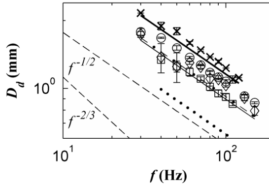
Figure 4: Drop diameter depending on the forcing frequency: ( \square ) D_p = 0.11 mm, q = 2.2 \mu\text{L.s}^{-1} , ( \diamond ) D_p = 0.32 mm, q = 6.5 \mu\text{L.s}^{-1} , ( \circ ) D_p = 0.35 mm, q = 6.9 \mu\text{L.s}^{-1} , ( \times ) D_p = 0.75 mm, q = 10.1 \mu\text{L.s}^{-1} . Estimates from eq. (9): D_p = 0.11 mm (dotted line), D_p = 0.32 mm (dash-dotted line), D_p = 0.35 mm (solid line), D_p = 0.75 mm (thick solid line).
