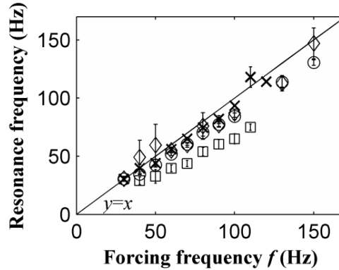
Figure 6: Calculated mode 1 resonance frequency [5] versus set experimental frequency: (□) D_p = 0.11 mm, q = 2.2 \mu\text{L.s}^{-1} , (◇) D_p = 0.32 mm, q = 6.5 \mu\text{L.s}^{-1} , (○) D_p = 0.35 mm, q = 6.9 \mu\text{L.s}^{-1} , (×) D_p = 0.75 mm, q = 10.1 \mu\text{L.s}^{-1} .
