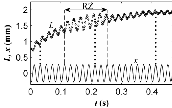
Figure 5: (◊) Drop length L , capillary displacement x (solid line), approximate boundaries of the resonance zone RZ (dashed line), phase shift estimation guidelines (dotted line): f = 50 Hz, D_p = 0.32 mm, A_{pp} = 0.56 mm < A_{th} = 0.88 mm, q = 4.3 \mu\text{L}\cdot\text{s}^{-1} .
