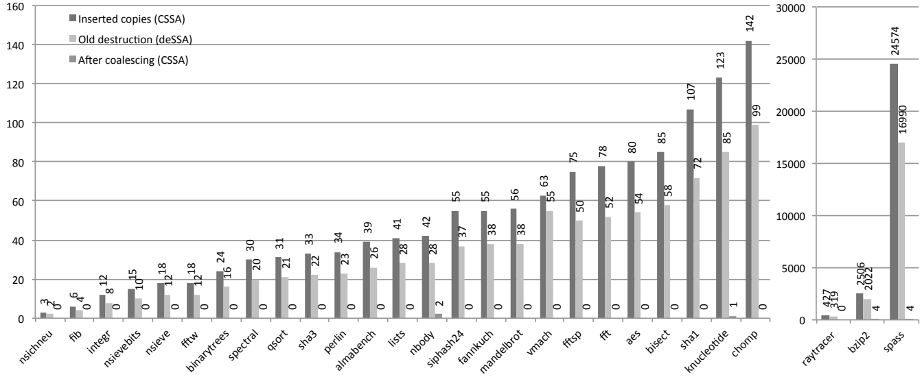
Figure 6: Coalescing results
