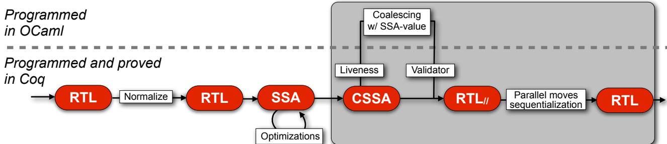
Figure 1: Overview of our SSA middle-end and SSA destruction (in grey)
