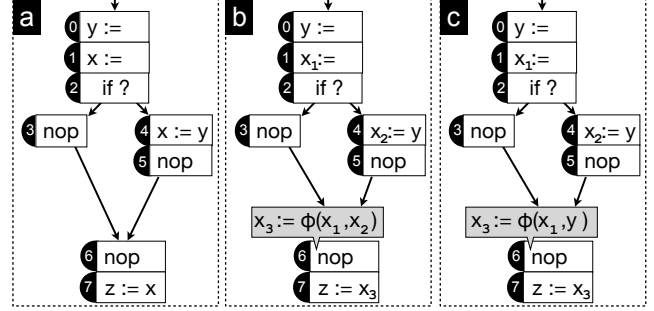
Figure 2: Example programs. Program a) is the initial normalized RTL program, Program b) is the SSA version and Program c) is obtained by propagating the copy at node 4 to node 6.
