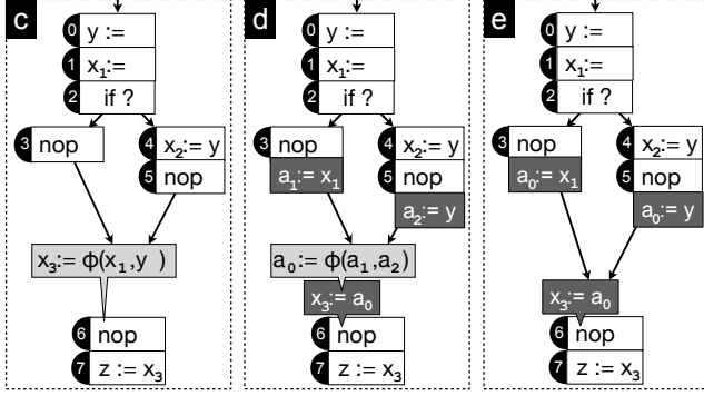
Figure 3: Example programs. Program c) is an optimized SSA program, Program d) is obtained by conversion to CSSA and Program e) is obtained by eliminating \phi -functions.
