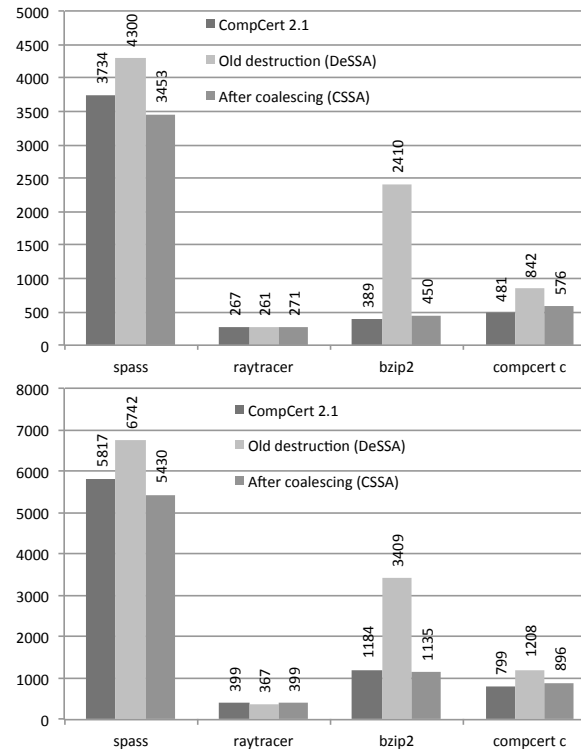
Figure 7: Spilling (top) and Reloading (bottom)
