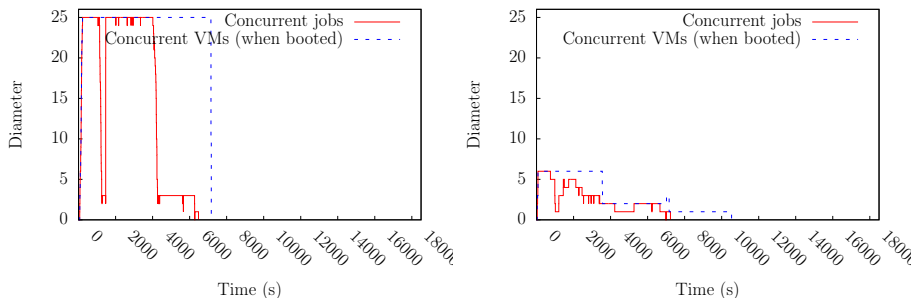
Figure 6: 3x3 executions on icps-cloud with ASAP (left) and AFAP (right)
