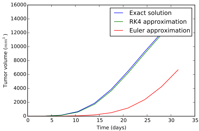
Figure 70: Euler approximation and RK4 approximation for h = 3.5
