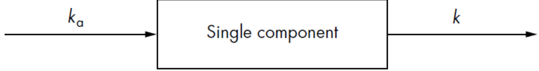
Figure 17: Unicompartamental model (absorption rate k_a and elimination rate k )
